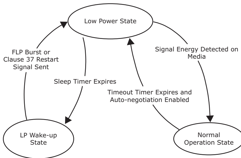
FIGURE 3-7: ACTIPHY STATE DIAGRAM
