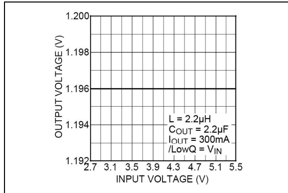
FIGURE 2-5: Line Regulation.
