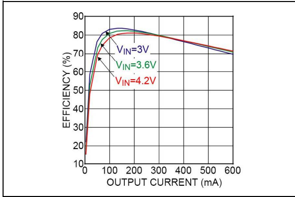
FIGURE 2-1: 1.2V OUT Efficiency.
