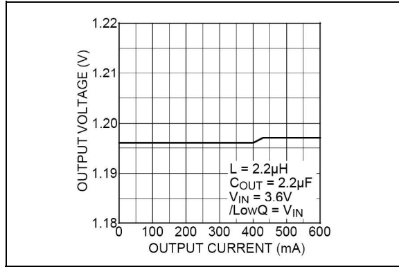
FIGURE 2-4: Load Regulation.
