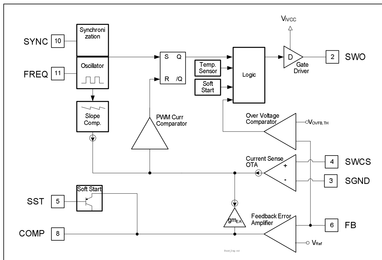
Figure 3 Boost regulator block diagram
