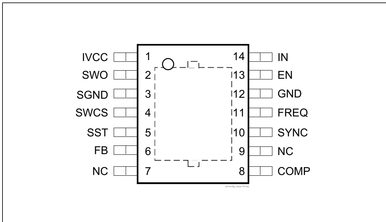
Figure 2 Pin assignment
