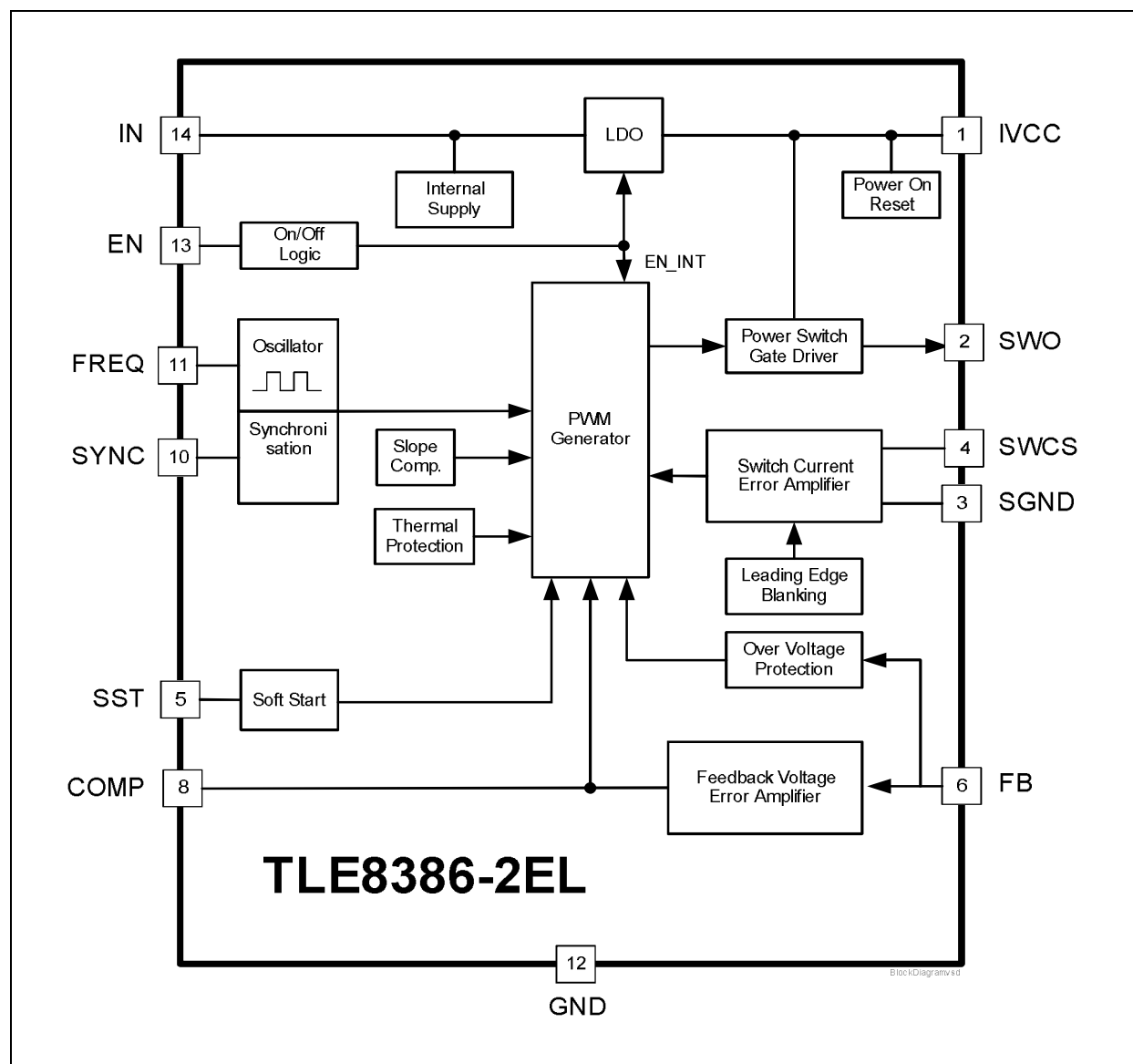
Figure 1 Block diagram
