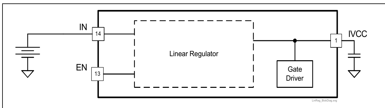
Figure 7 Voltage regulator block diagram and simplified application circuit
