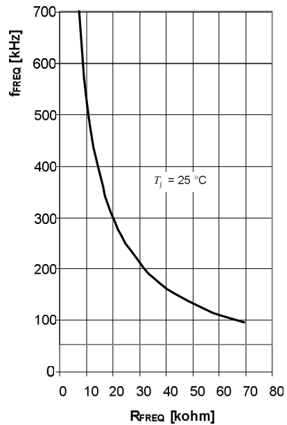
Switching frequency f_{SW} versus frequency select resistor to GND R_{FREQ}
