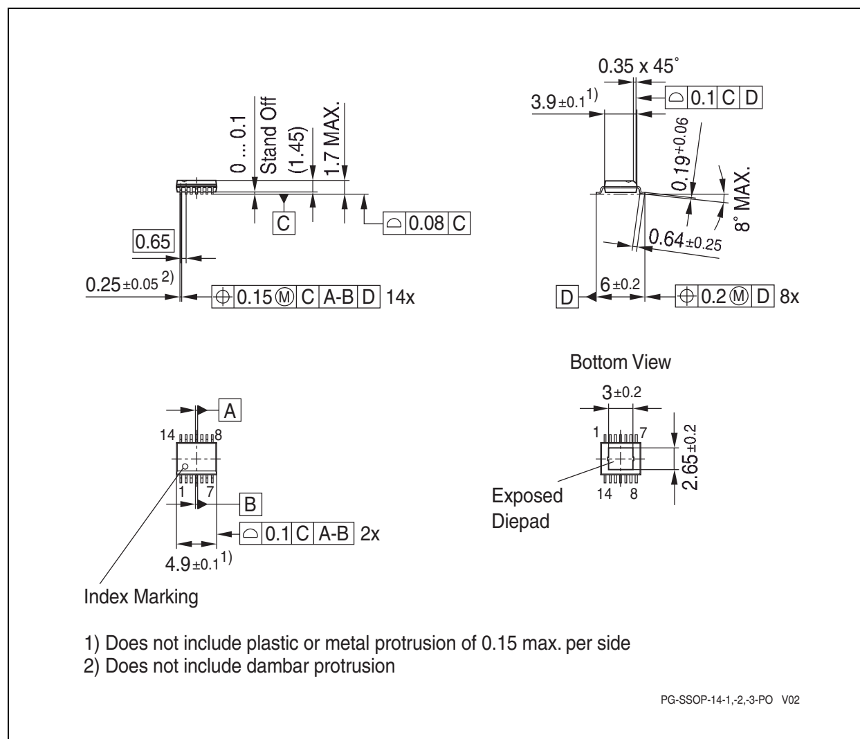
Figure 11 PG-SSOP-14 1)
