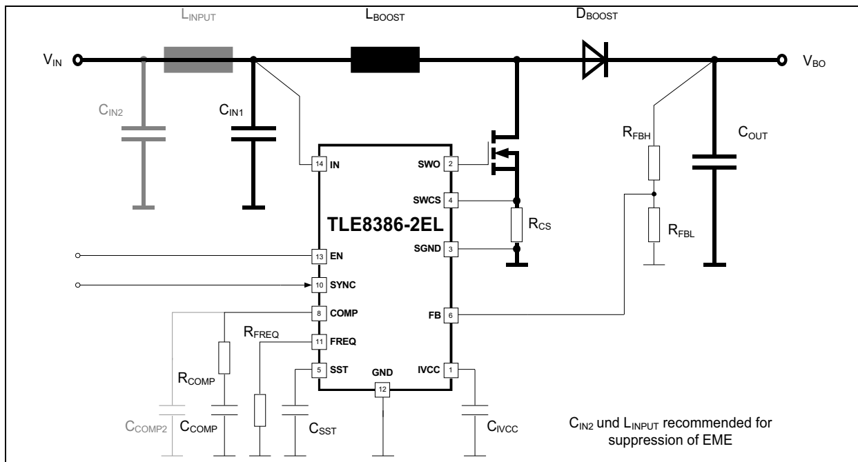
Figure 8 Boost converter application circuit
