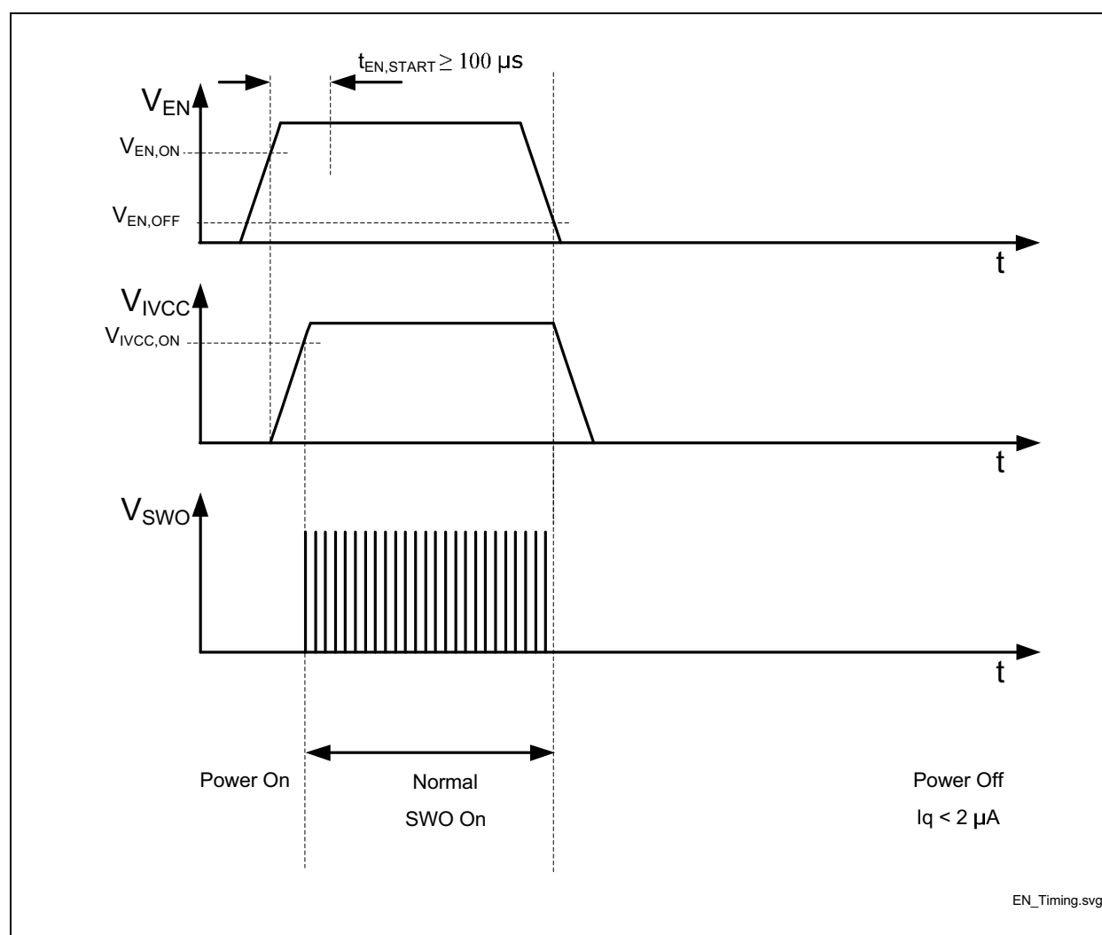
Figure 6 Enable timing diagram
