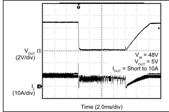
FIGURE 2-60: Output Recovery from Short-Circuit.
