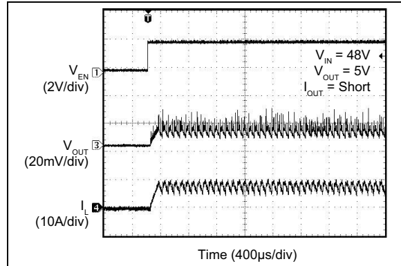
FIGURE 2-58: Enabled into Short-Circuit.
