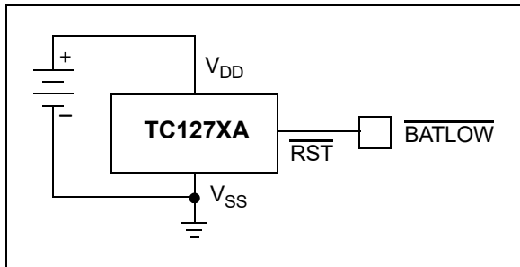
FIGURE 5-2: Battery Voltage Monitor.
