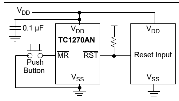
FIGURE 4-3: Typical Open-Drive Application Circuit.
