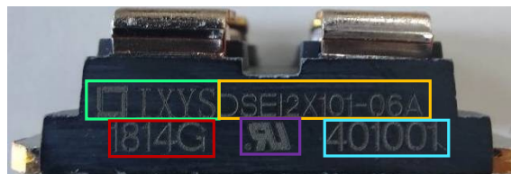
Figure 3: SOT-227B marking description
