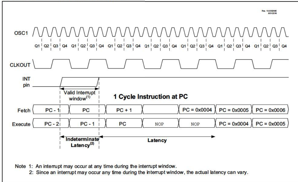
FIGURE 10-2: INTERRUPT LATENCY
