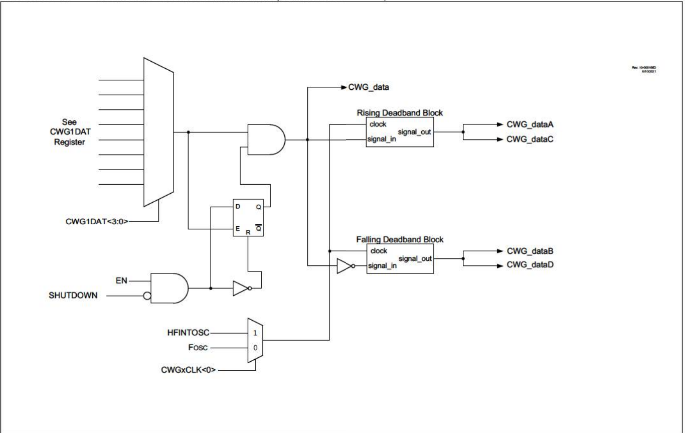
FIGURE 30-1: SIMPLIFIED CWG BLOCK DIAGRAM (HALF-BRIDGE MODE)
