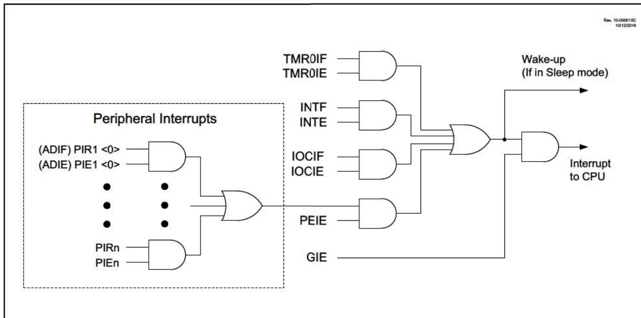
FIGURE 10-1: INTERRUPT LOGIC
