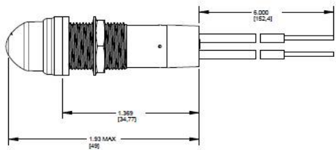
Old Part (Before Inset Modification)
