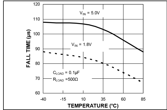
FIGURE 2-28: Output Fall Time vs. Temperature.
