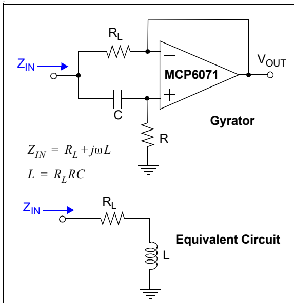
FIGURE 4-8: Gyrator.
