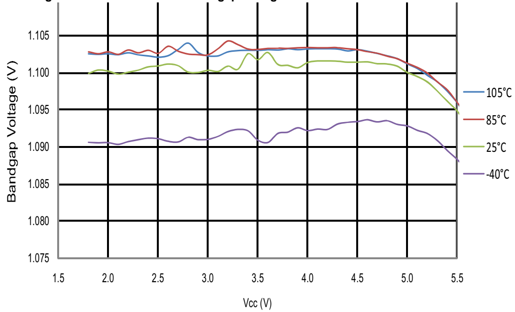
Figure 31-35. ATmega48PB/88PB: Calibrated Bandgap Voltage vs. Vcc
