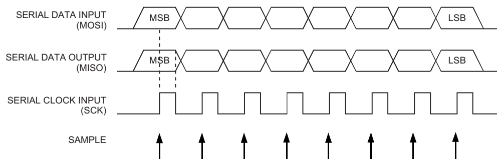
Figure 29-9. Serial Programming Waveforms
