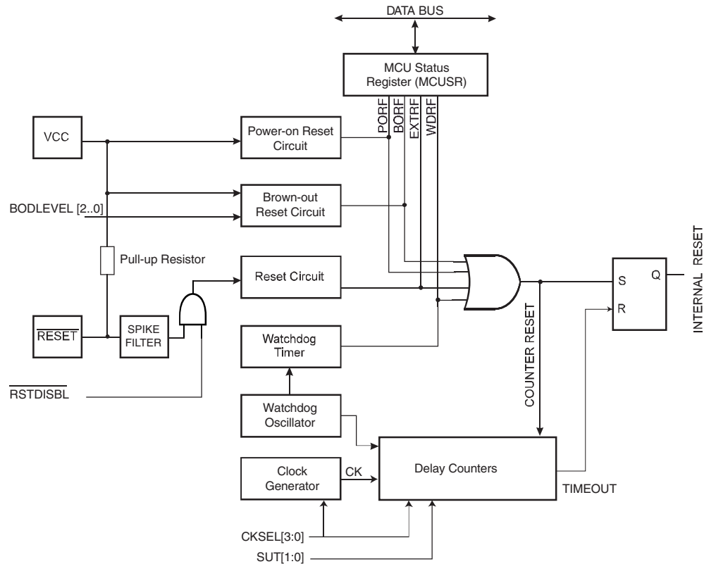
Figure 12-1. Reset Logic
