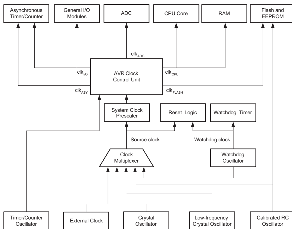
Figure 10-1. Clock Distribution
