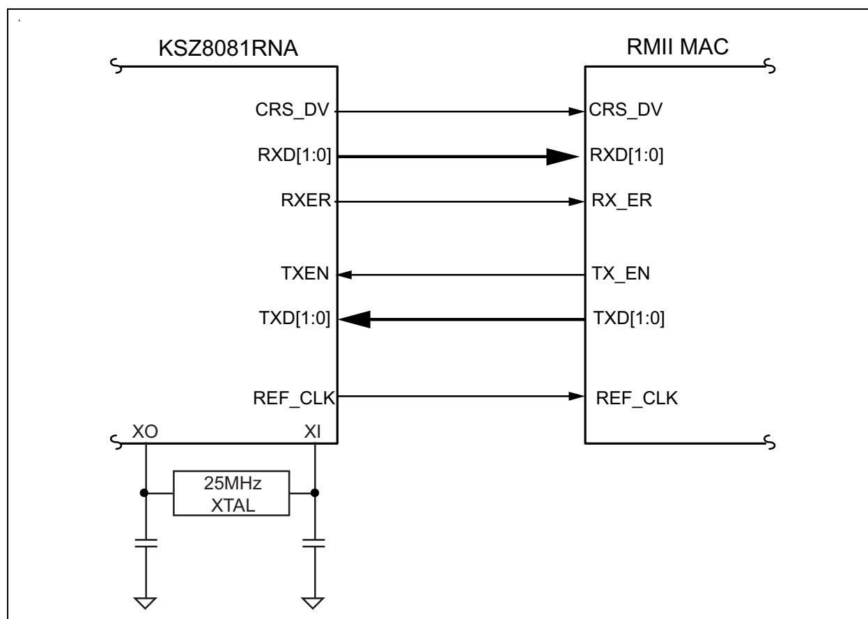
FIGURE 3-2: KSZ8081RNA RMII INTERFACE (RMII - 25 MHZ CLOCK MODE)
