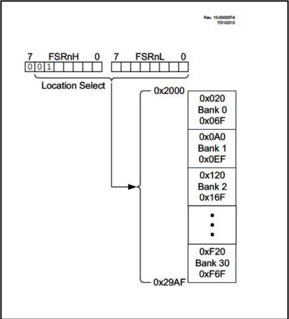
FIGURE 3-11: LINEAR DATA MEMORY MAP
