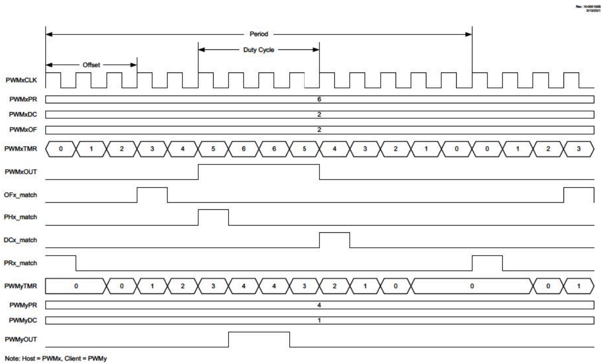
FIGURE 22-12: OFFSET MATCH ON INCREMENTING TIMER TIMING DIAGRAM
