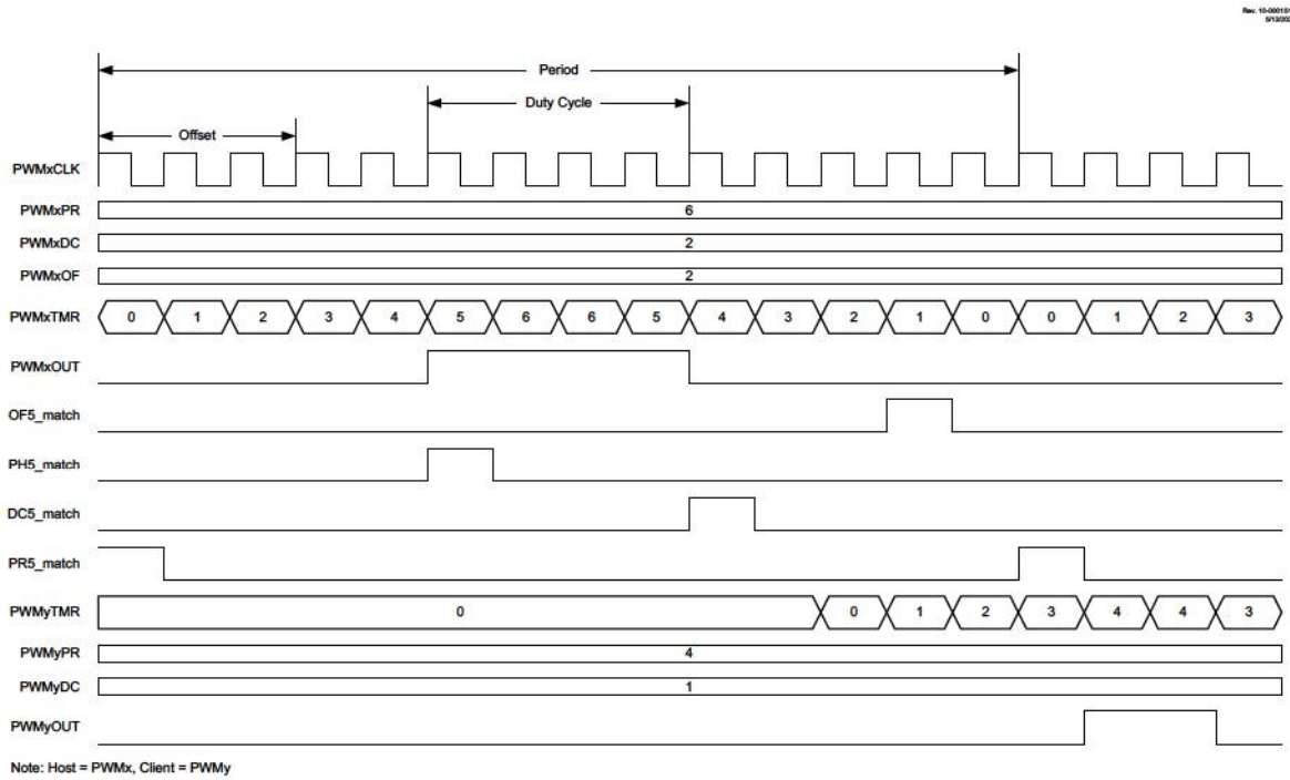
FIGURE 22-13: OFFSET MATCH ON DECREMENTING TIMER TIMING DIAGRAM
