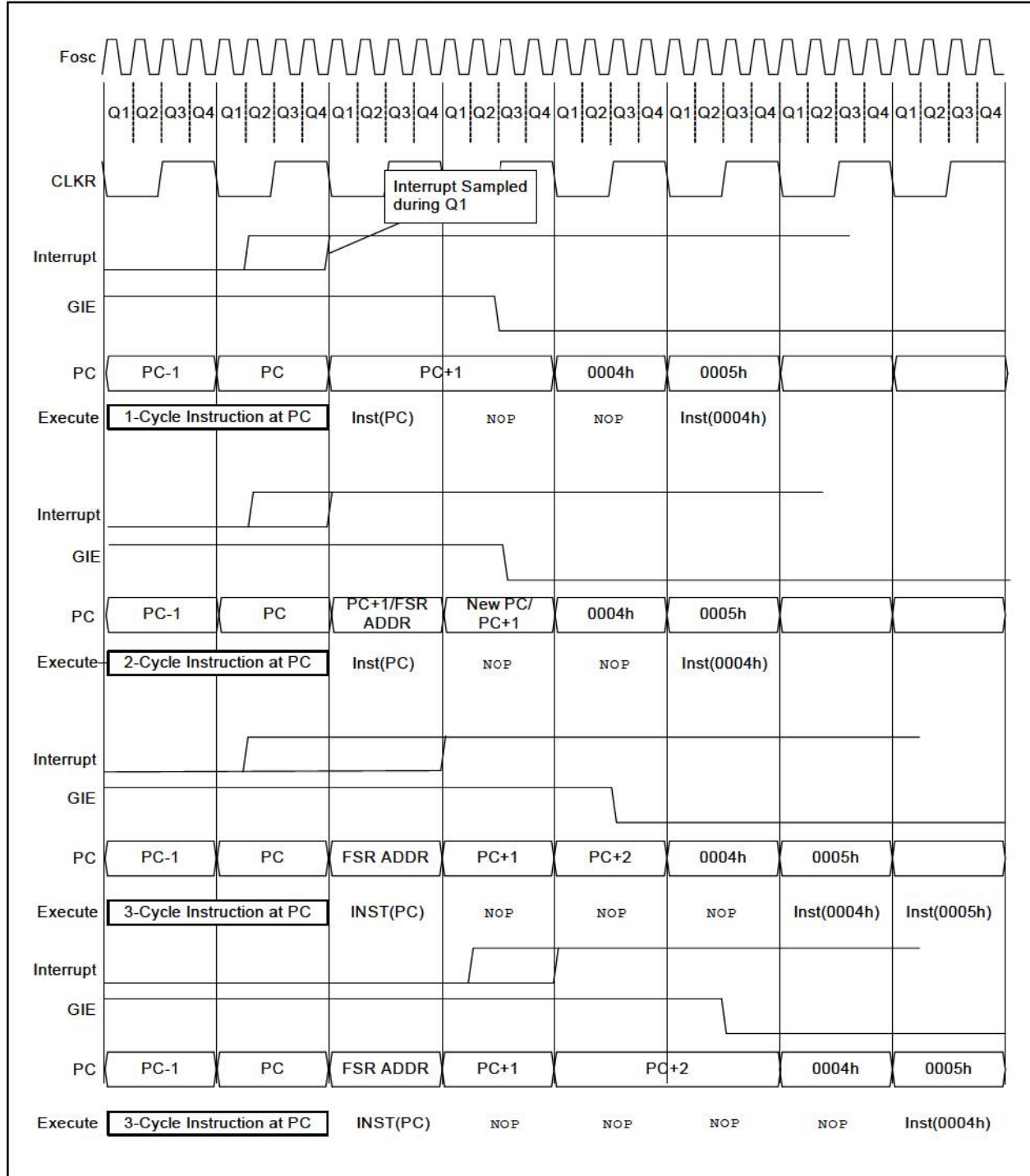
FIGURE 7-2: INTERRUPT LATENCY
