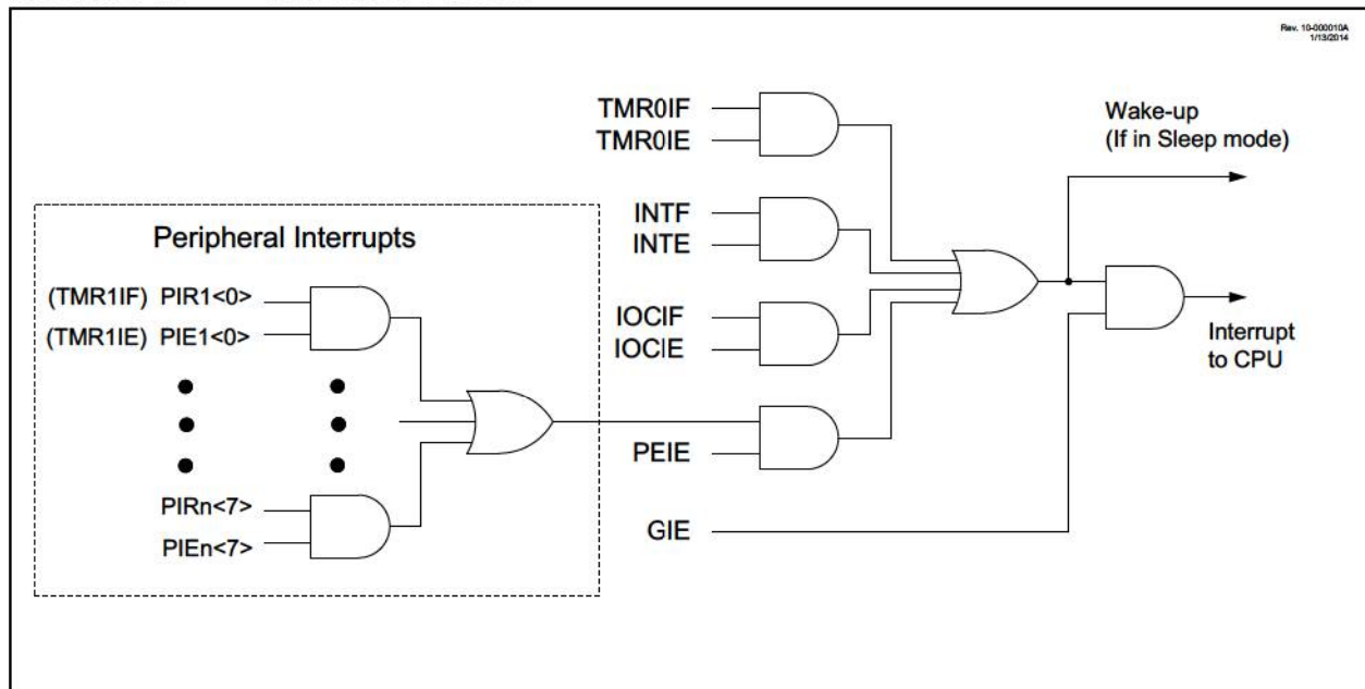
FIGURE 7-1: INTERRUPT LOGIC
