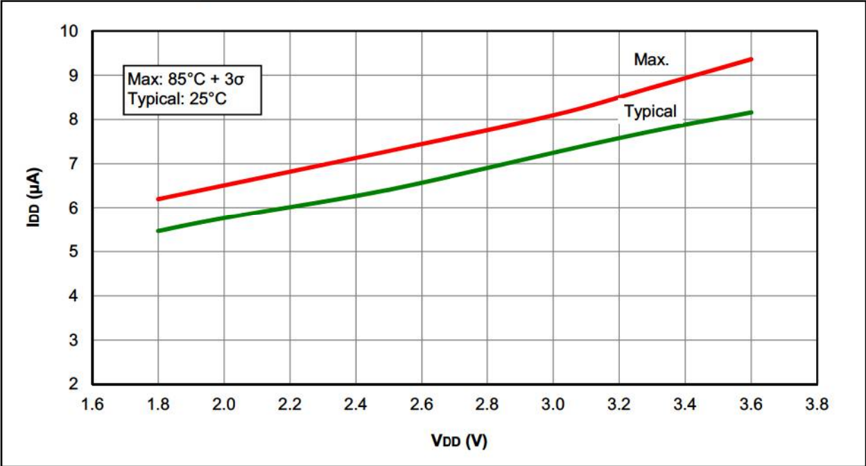
FIGURE 27-13: I_{DD} , LFINTOSC, F_{osc} = 31\text{ kHz} , PIC12LF1571/2 ONLY
