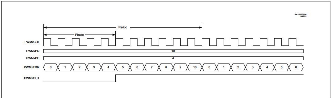
FIGURE 22-5: SET ON MATCH PWM MODE TIMING DIAGRAM
