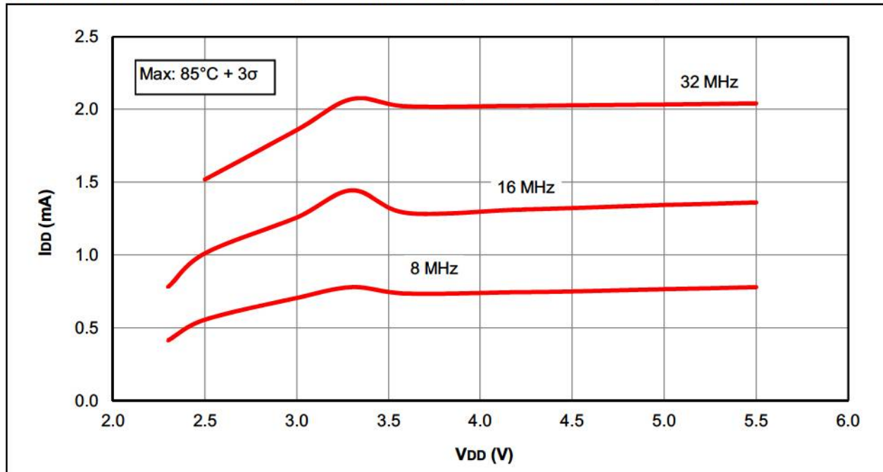
FIGURE 27-12: I DD MAXIMUM, EC OSCILLATOR, HIGH POWER MODE, PIC12F1571/2 ONLY
