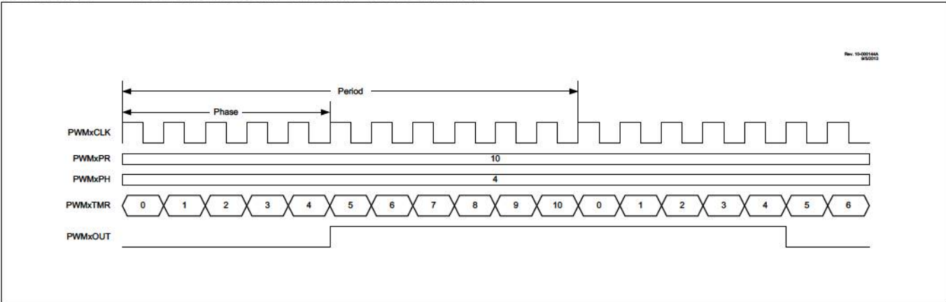
FIGURE 22-6: TOGGLE ON MATCH PWM MODE TIMING DIAGRAM
