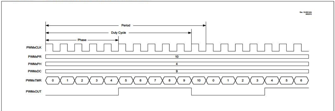
FIGURE 22-4: STANDARD PWM MODE TIMING DIAGRAM
