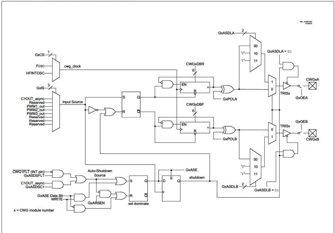
FIGURE 23-1: SIMPLIFIED CWG BLOCK DIAGRAM
