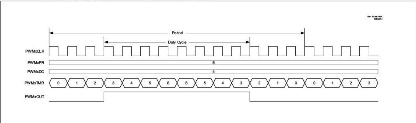
FIGURE 22-7: CENTER-ALIGNED PWM MODE TIMING DIAGRAM
