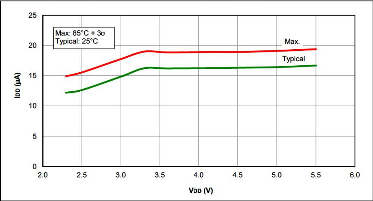
FIGURE 27-14: I_{DD} , LFINTOSC, F_{osc} = 31\text{ kHz} , PIC12F1571/2 ONLY
