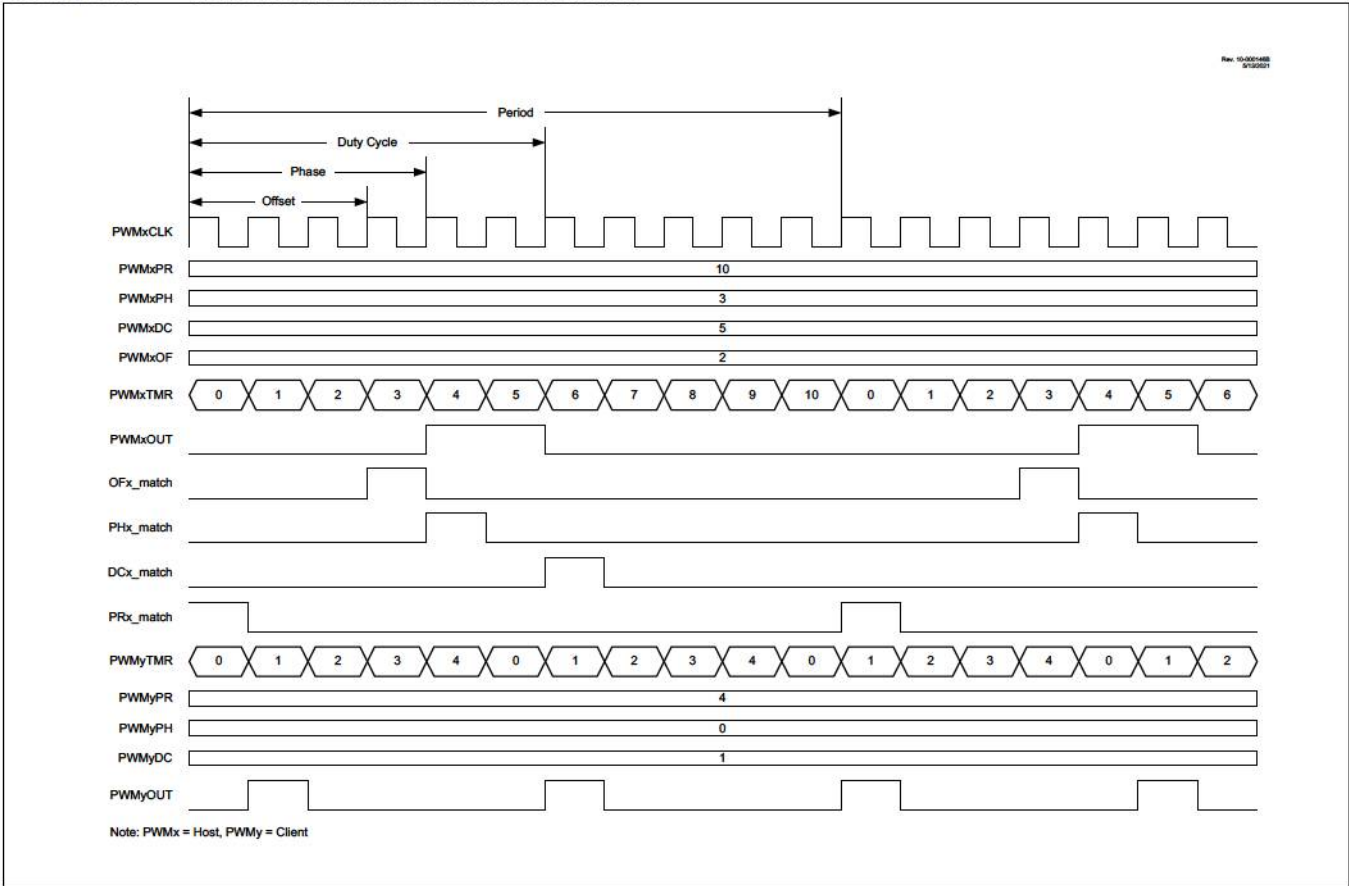
FIGURE 22-8: INDEPENDENT RUN MODE TIMING DIAGRAM
