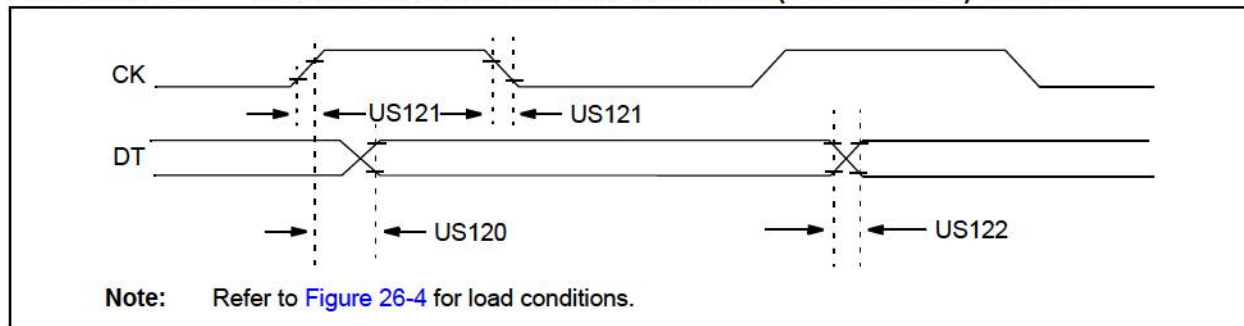
FIGURE 26-13: USART SYNCHRONOUS TRANSMISSION (HOST/CLIENT) TIMING
