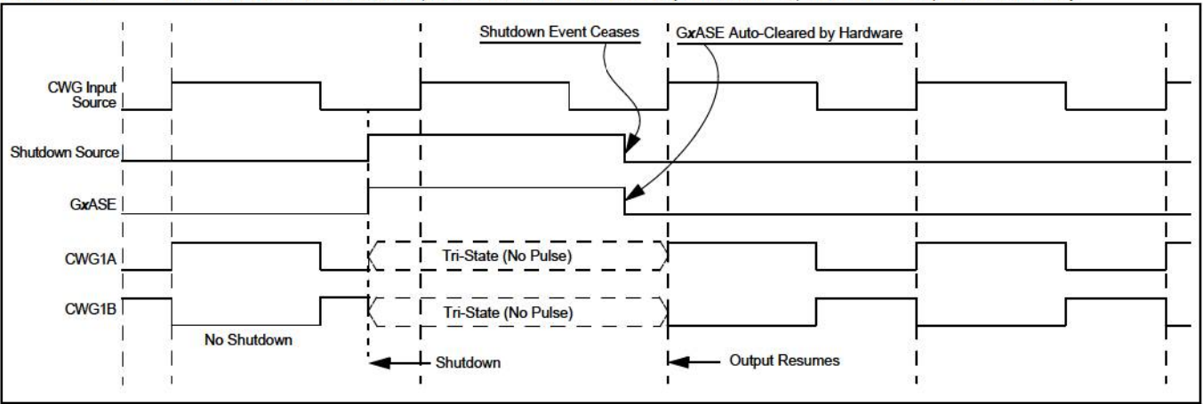
FIGURE 23-6: SHUTDOWN FUNCTIONALITY, AUTO-RESTART ENABLED (GxARSEN = 1, GxASDLA = 01, GxASDLB = 01)
