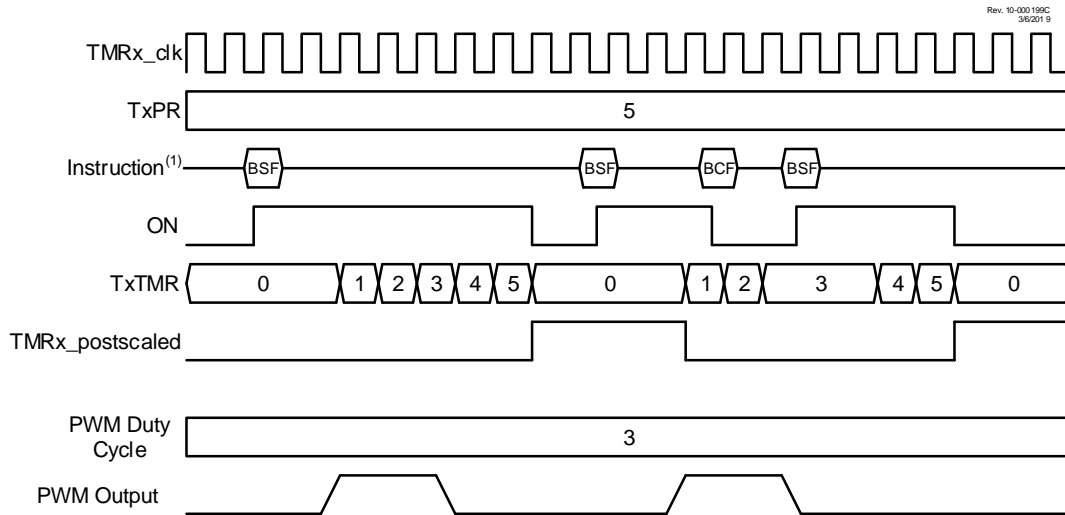
Figure 21-7. Software Start One Shot Mode Timing Diagram (MODE = 'b01000)
