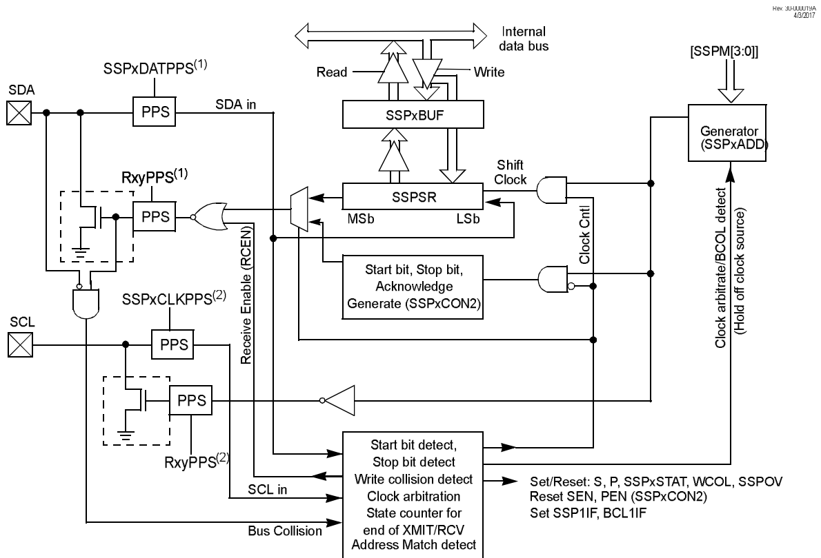
Figure 25-9. MSSP Block Diagram (I 2 C Host Mode)
