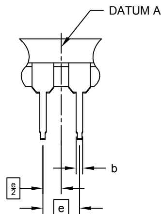
ALTERNATE LEAD DESIGN (NOTE 5)
