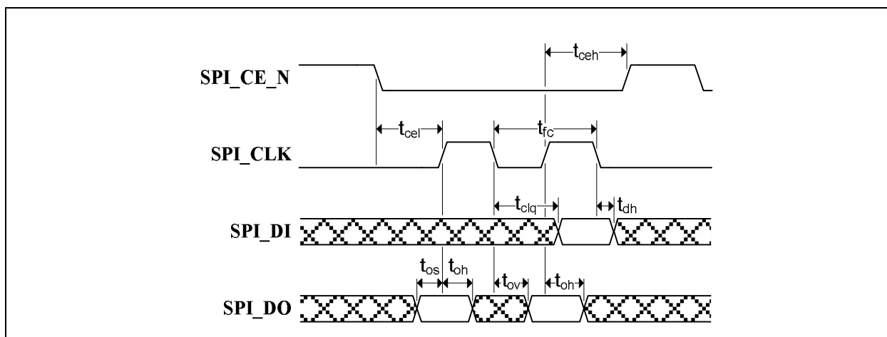
FIGURE 10-5: SPI TIMING
