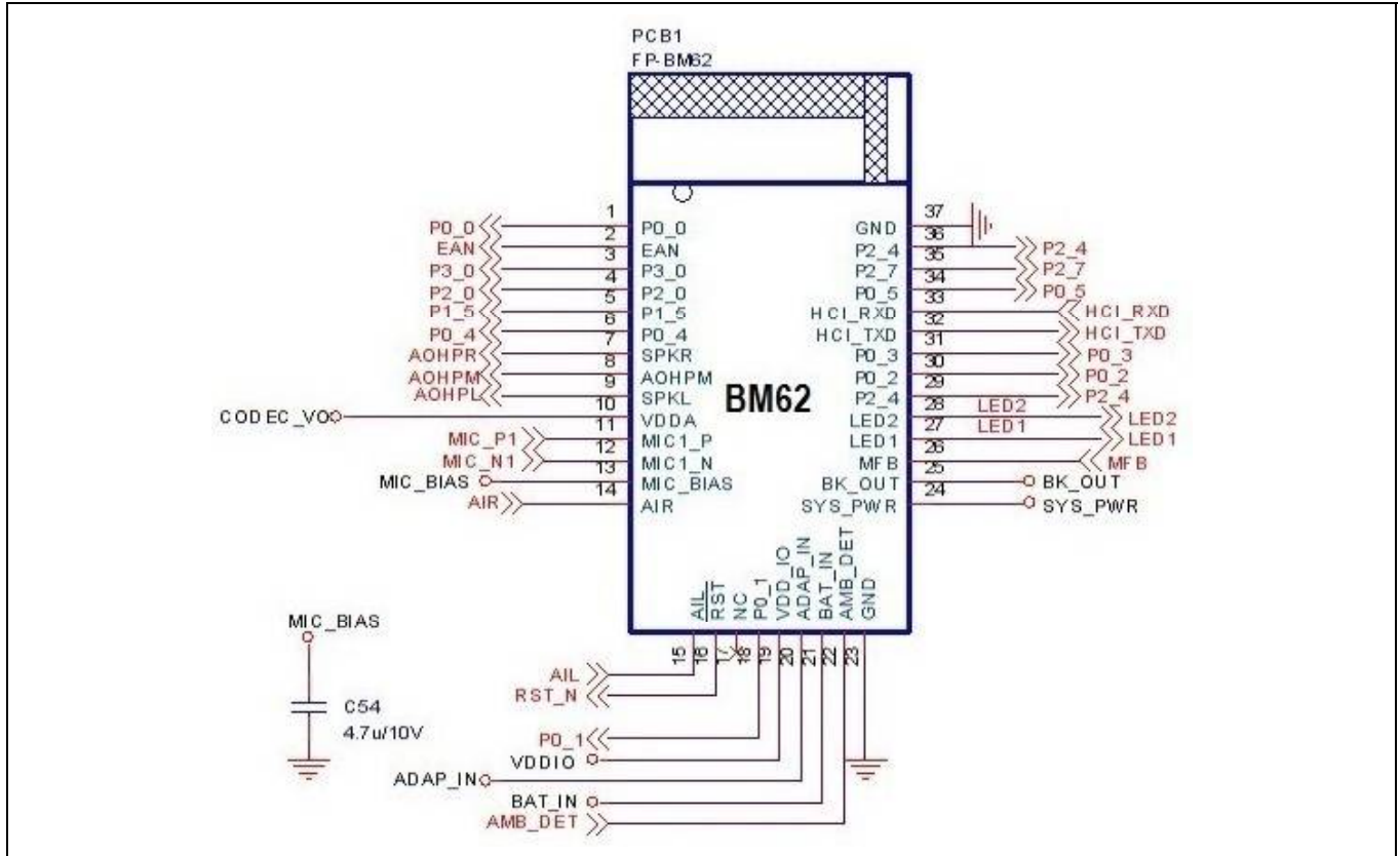
FIGURE 5-14: BM62 REFERENCE CIRCUIT FOR STEREO HEADSET APPLICATION
