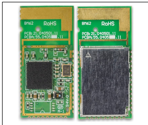
FIGURE 1: BM62 MODULE
