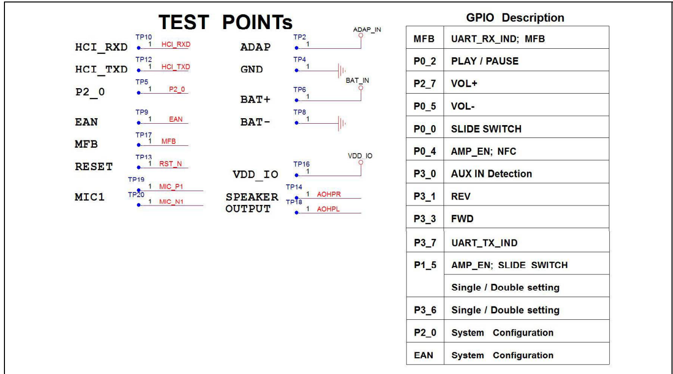
FIGURE 5-19: BM64 REFERENCE CIRCUIT FOR STEREO HEADSET APPLICATION
