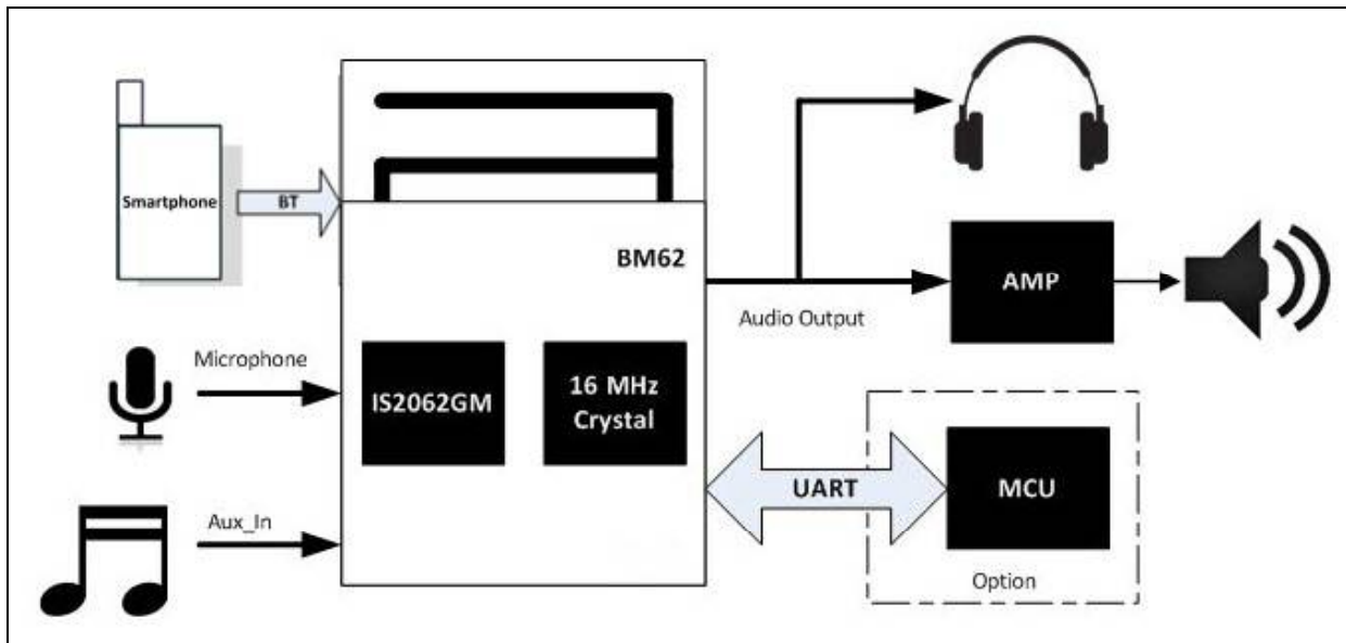
FIGURE 1-1: SINGLE SPEAKER APPLICATION USING BM62 MODULE
