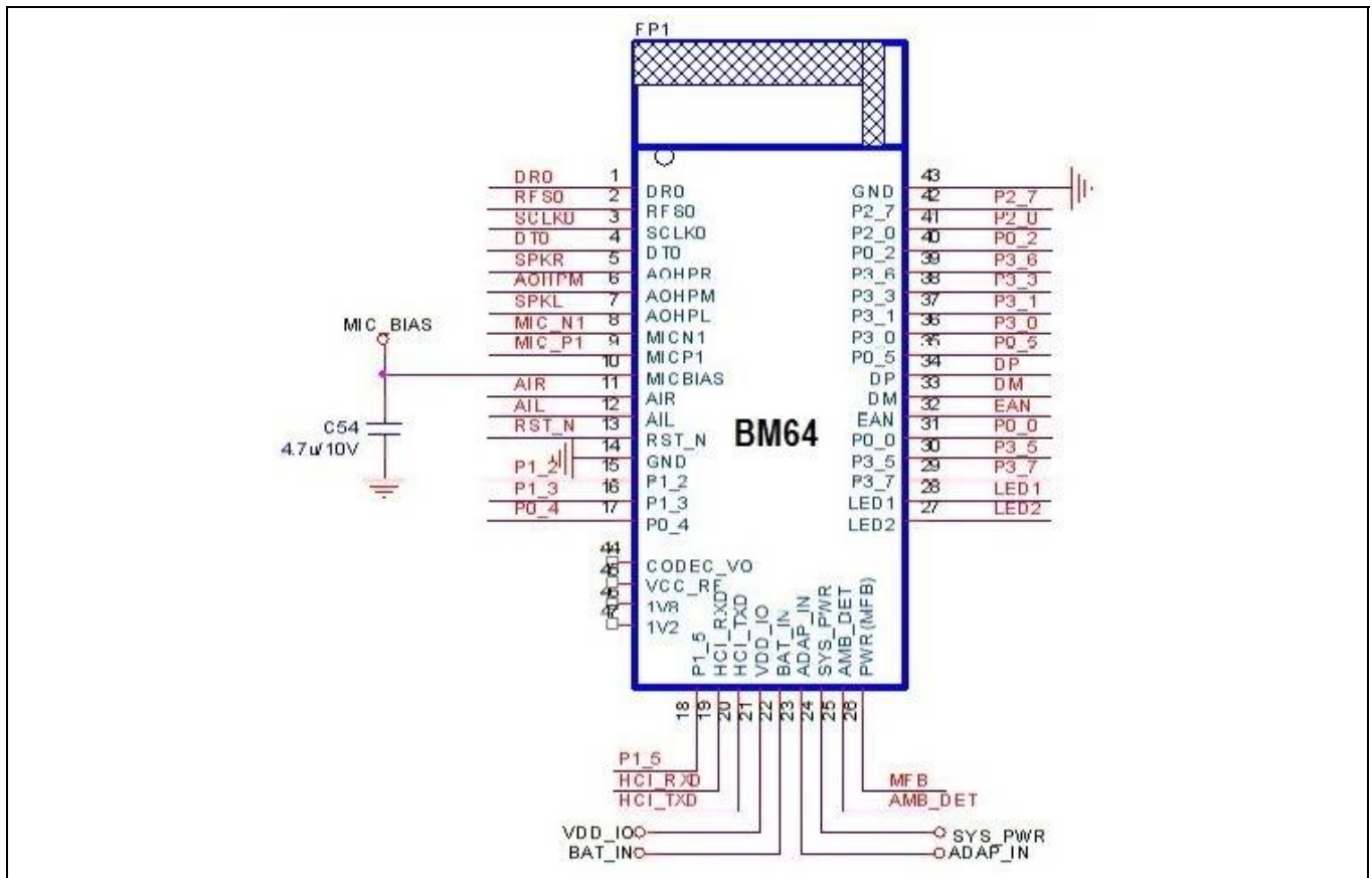
FIGURE 5-18: BM64 REFERENCE CIRCUIT FOR STEREO HEADSET APPLICATION
