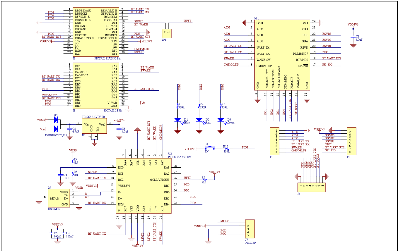
FIGURE 5-1: RN4020 TYPICAL APPLICATION SCHEMATICS
