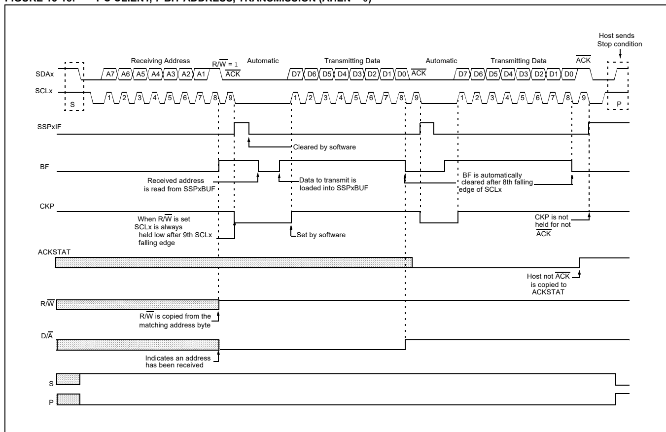
FIGURE 15-18: I 2 C CLIENT, 7-BIT ADDRESS, TRANSMISSION (AHEN = 0)
