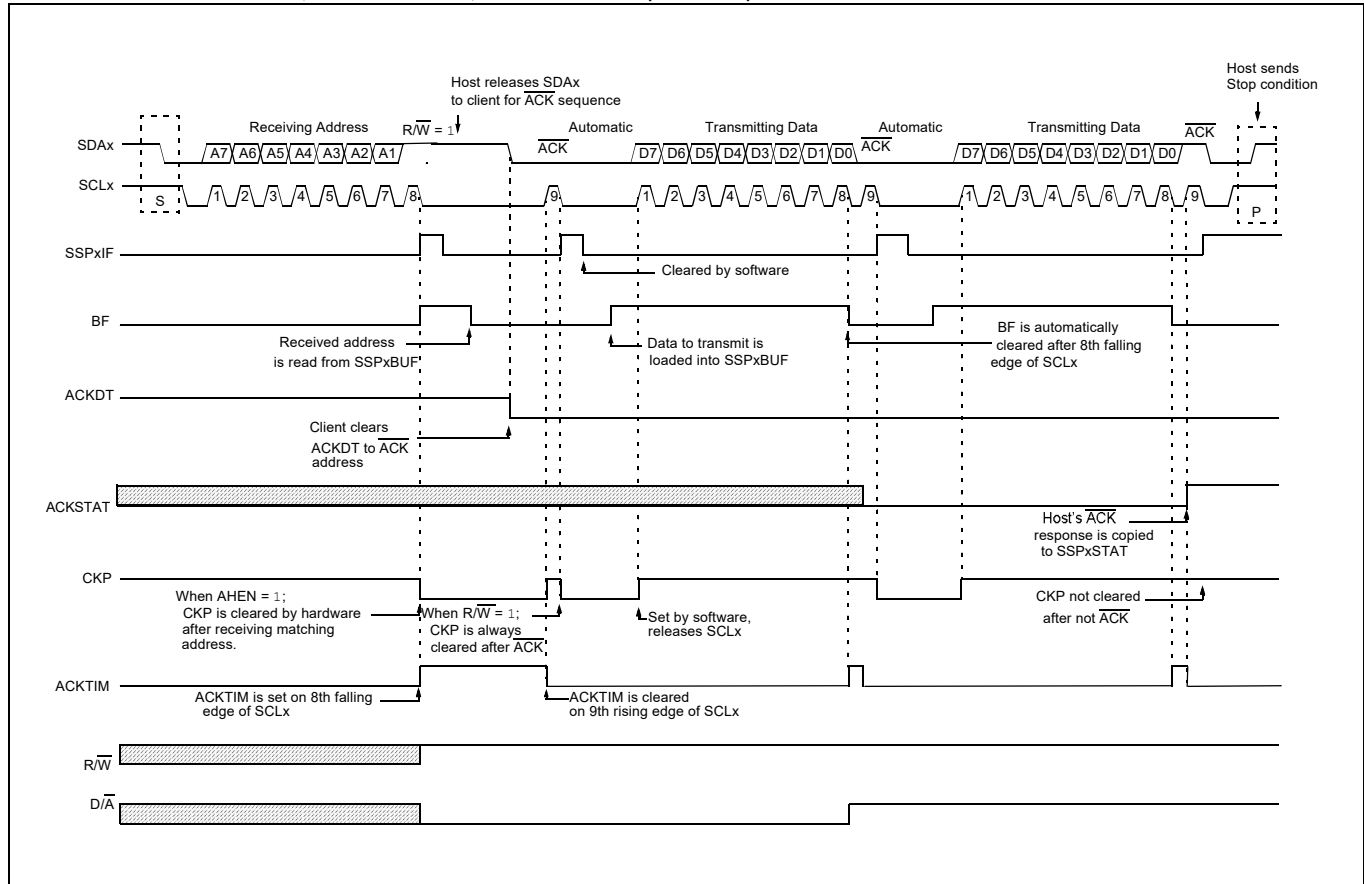
FIGURE 15-19: I 2 C CLIENT, 7-BIT ADDRESS, TRANSMISSION (AHEN = 1)
