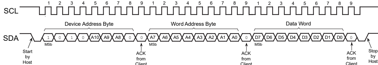
Figure 7-1. Byte Write
