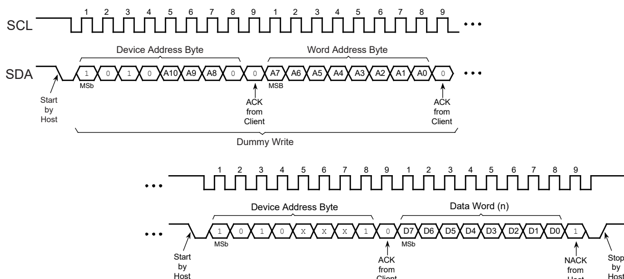
Figure 8-2. Random Read
