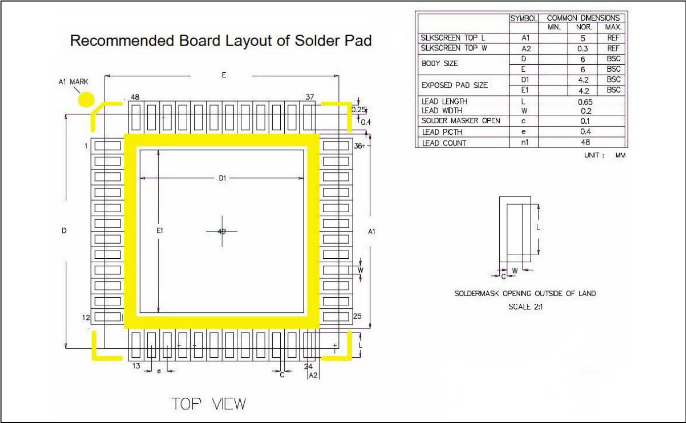
FIGURE 4-2: 48QFN, 6X6 MM FOOTPRINT INFORMATION (IS1870SF)
