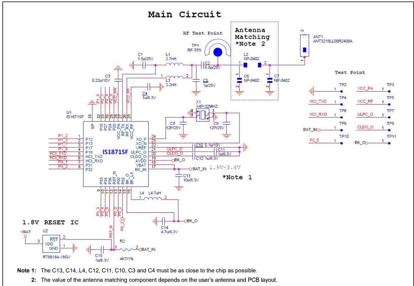
FIGURE A-3: IS1871 SOC APPLICATION CIRCUIT
