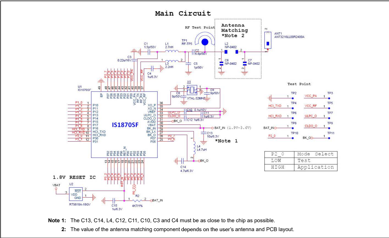
FIGURE A-1: IS1870 SOC APPLICATION CIRCUIT
