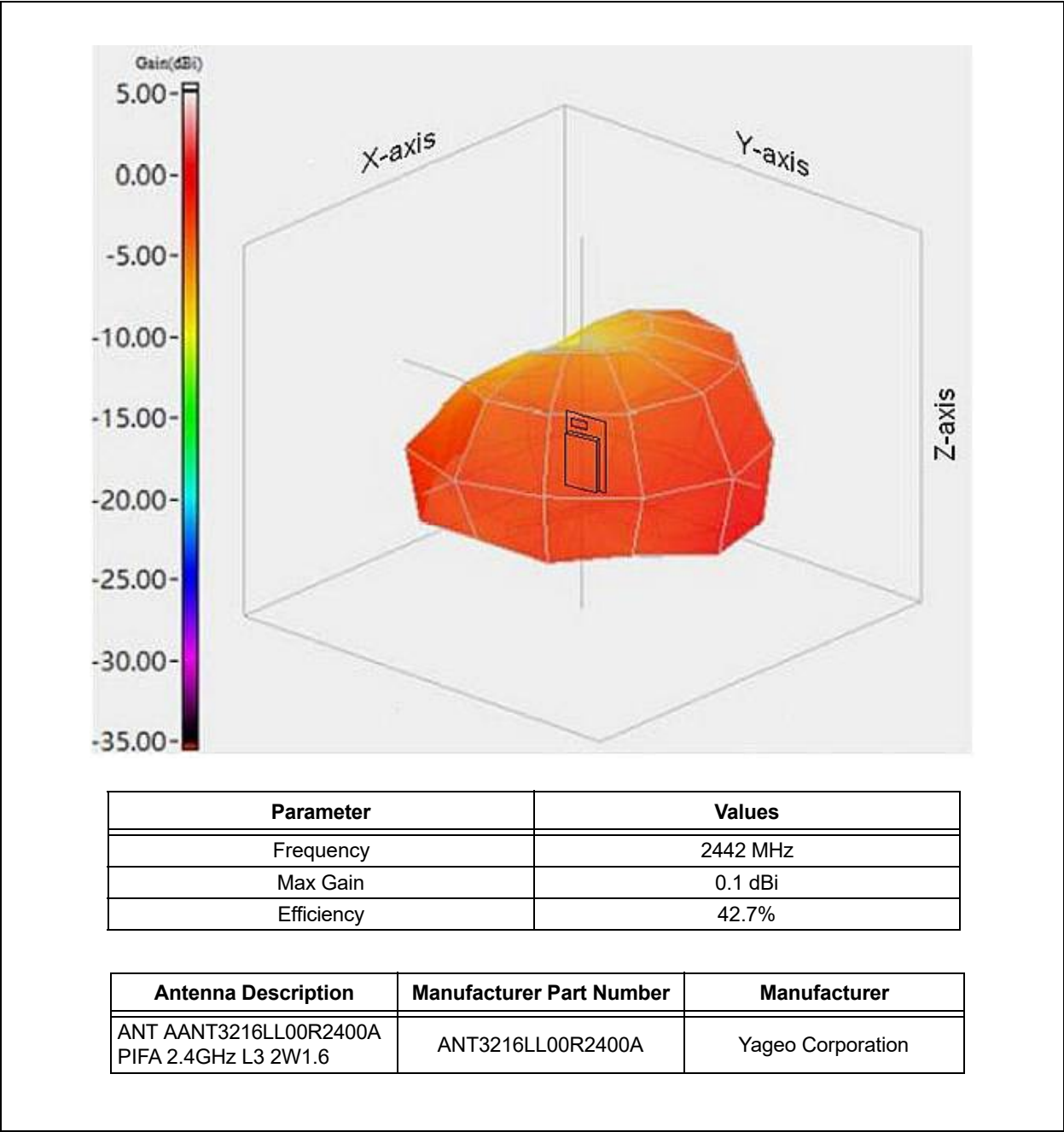
FIGURE 8-2: RN4871 ANTENNA PERFORMANCE
