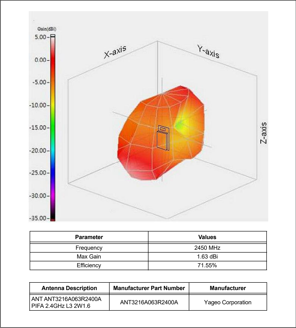
FIGURE 8-1: RN4870 ANTENNA PERFORMANCE
