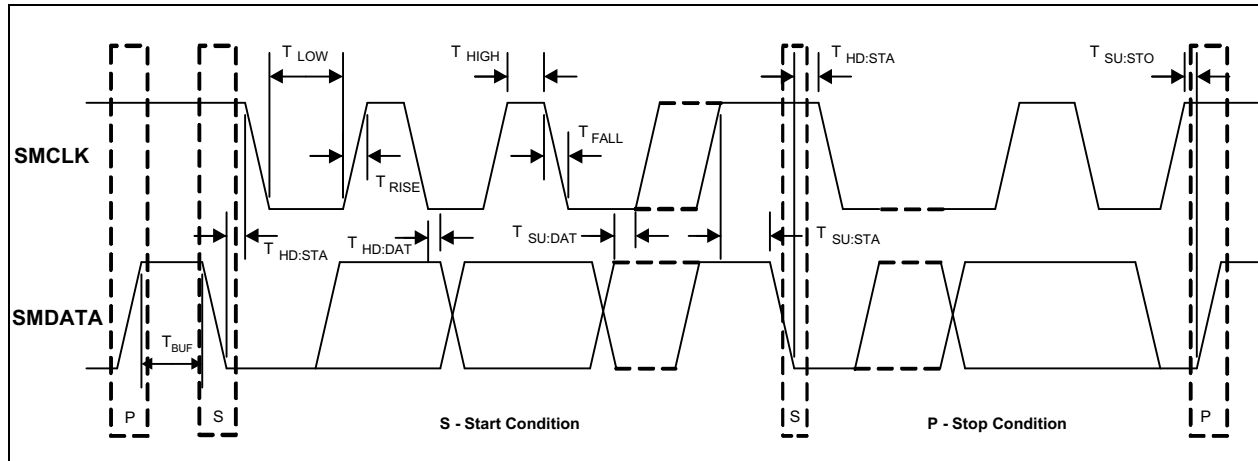
FIGURE 1-1: SMBus Timing.
