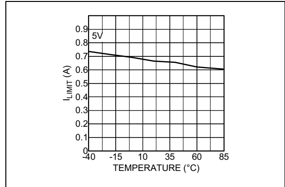
FIGURE 2-16: I LIMIT vs. Temperature (MIC20X5A).
