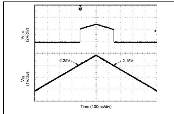
FIGURE 2-30: UVLO.
