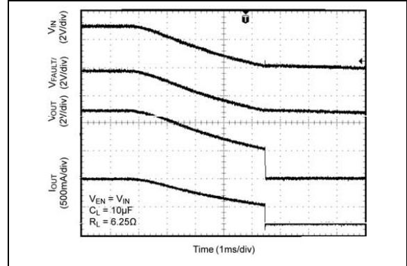
FIGURE 2-28: Turn-Off V_{IN} .
