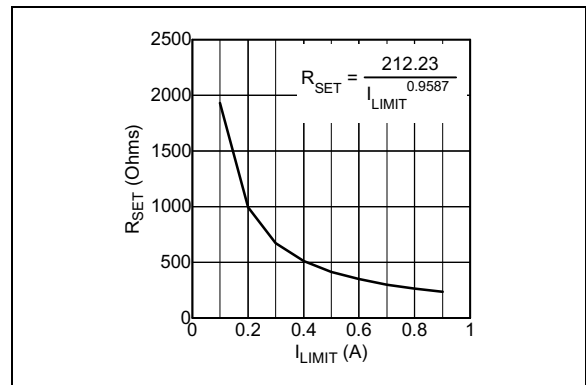
FIGURE 2-18: R SET vs I LIMIT (MIC20X9A).
