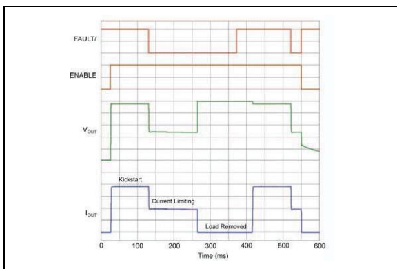
FIGURE 5-8: Kickstart.
