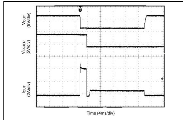
FIGURE 2-42: Kickstart Response Time 5A Over Load.
