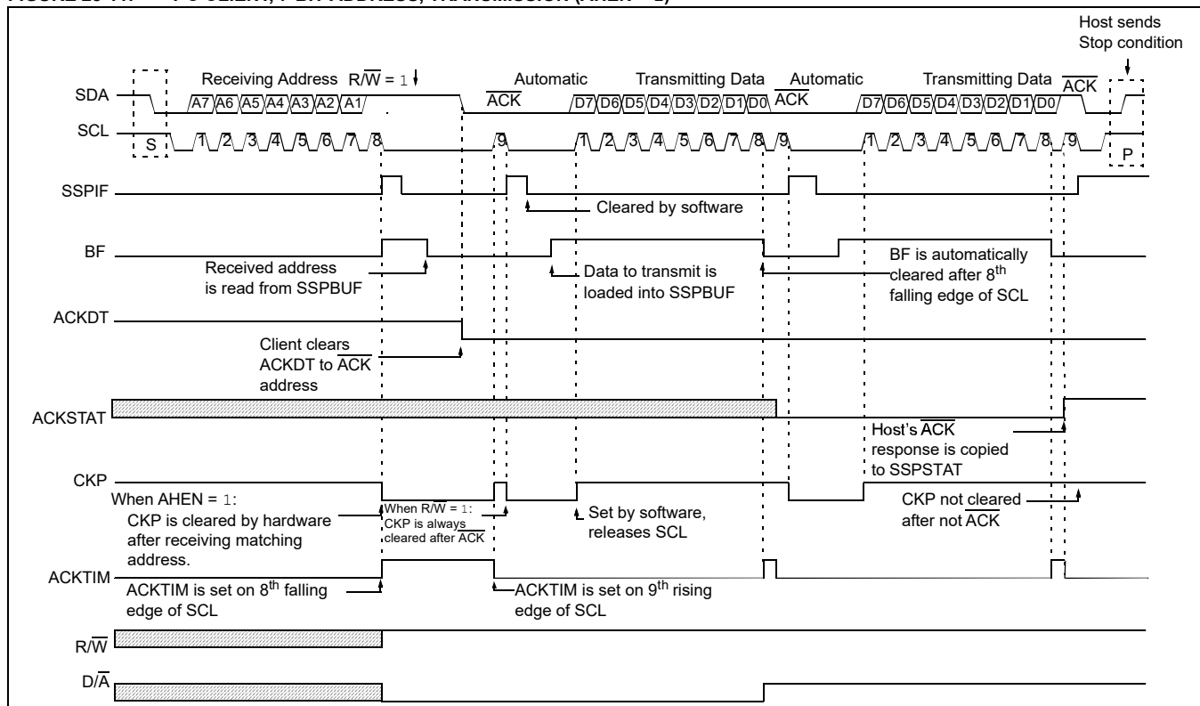
FIGURE 28-11: I 2 C CLIENT, 7-BIT ADDRESS, TRANSMISSION (AHEN = 1)
