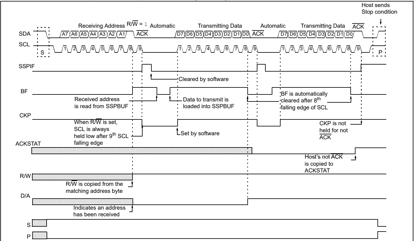
FIGURE 28-10: I 2 C CLIENT, 7-BIT ADDRESS, TRANSMISSION (AHEN = 0)
