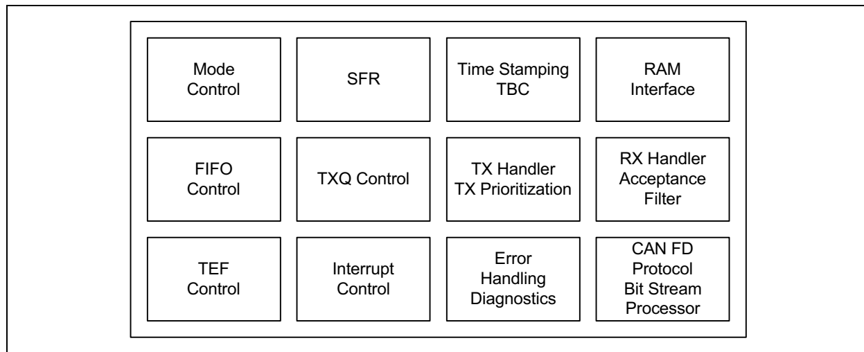
FIGURE 2-1: CAN FD CONTROLLER MODULE BLOCK DIAGRAM
