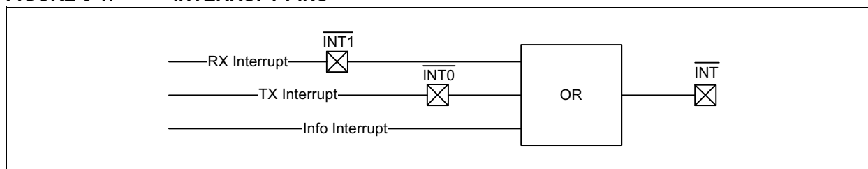
FIGURE 6-1: INTERRUPT PINS
