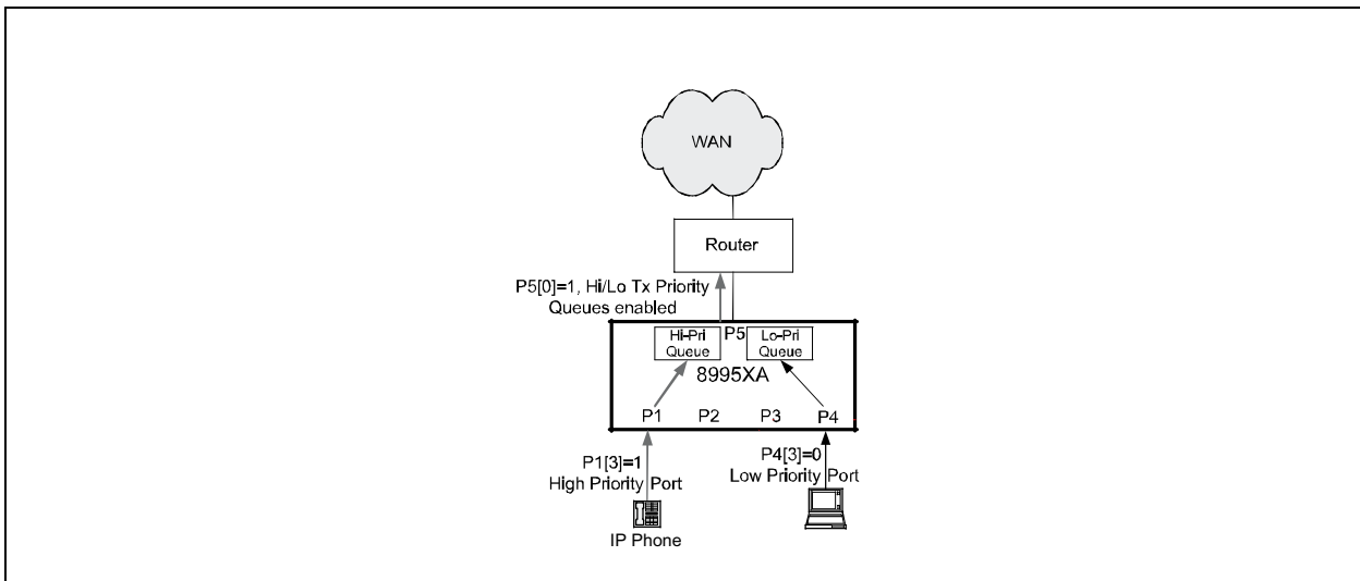
FIGURE 3-2: PORT-BASED PRIORITY
