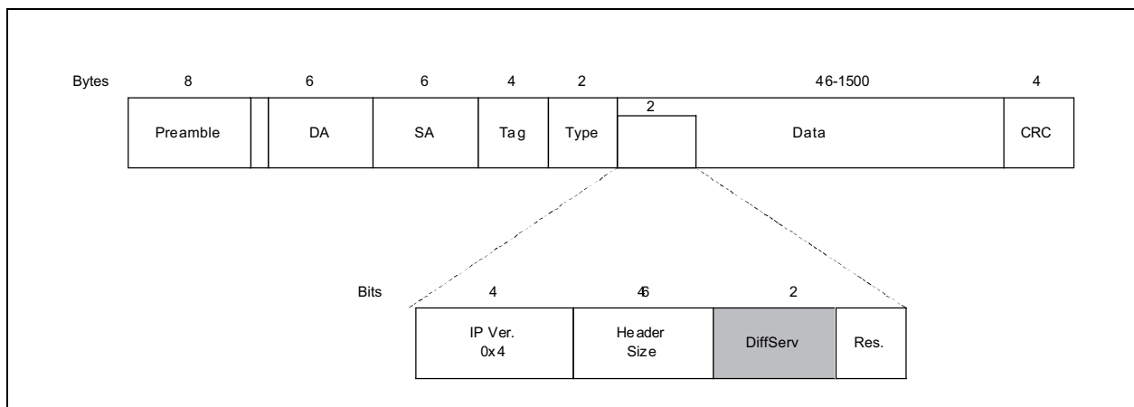
FIGURE 3-4: IPV4 PACKET
