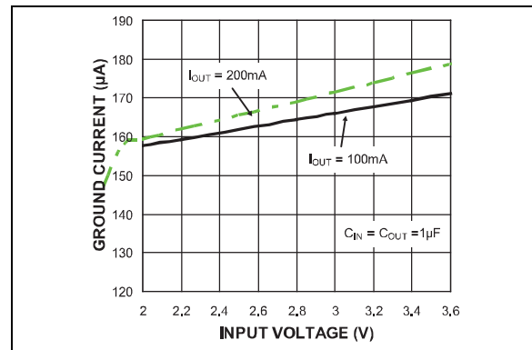
FIGURE 2-18: Ground Current vs. Input Voltage.
