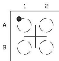
MIC94310 0.88 mm x 0.88 mm 4-Ball WLCSP (Top View)
