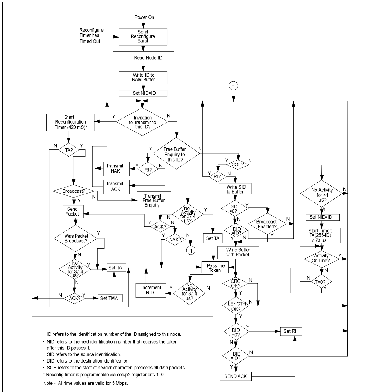
FIGURE 3-1: COM20020ID OPERATION
