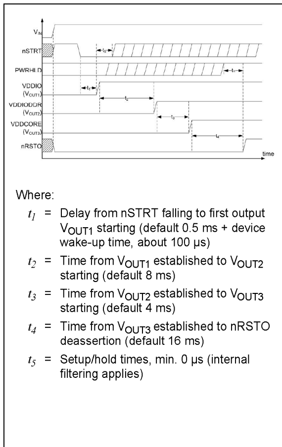
FIGURE 4-4: Start-Up from nSTRT Timing Diagram.
