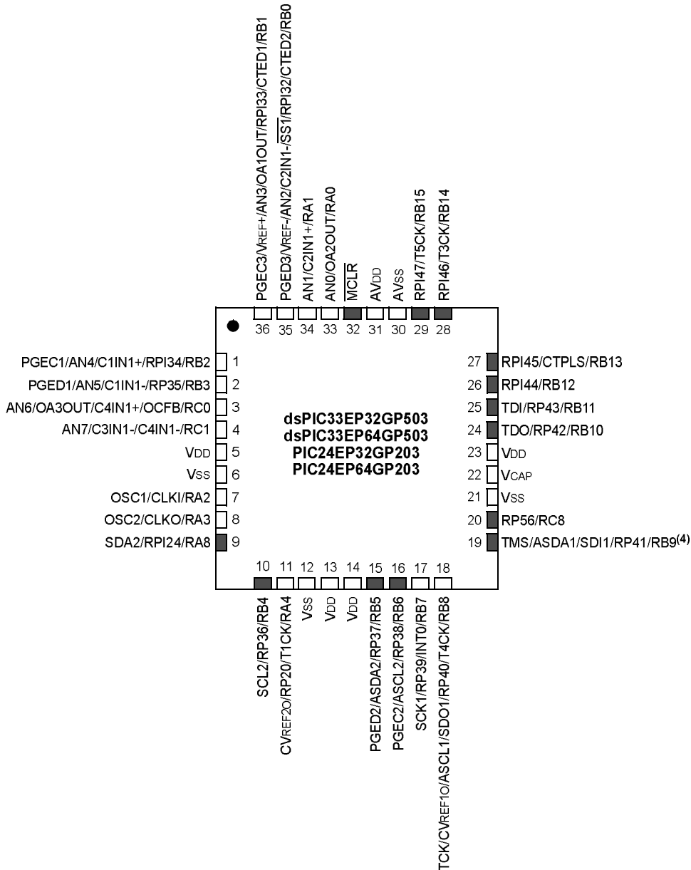
36-Pin UQFN (1,2,3)
