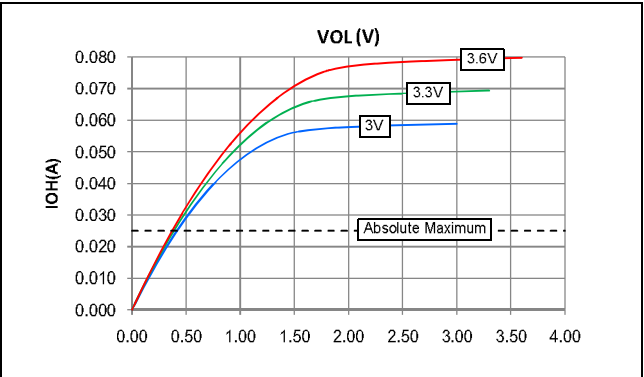
FIGURE 32-4: VOL – 8x DRIVER PINS
