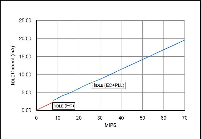
FIGURE 32-8: TYPICAL IDLE CURRENT @ VDD = 3.3V
