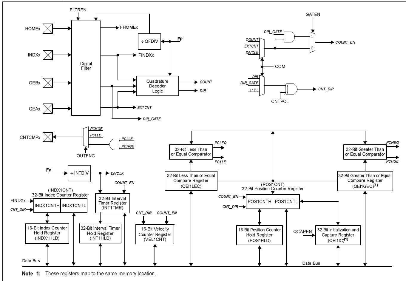
FIGURE 17-1: QE1 BLOCK DIAGRAM
