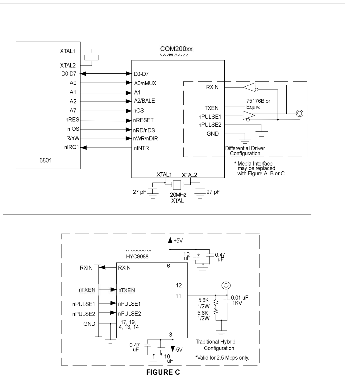
FIGURE 5-2: NON-MULTIPLEXED, 6801-LIKE BUS INTERFACE WITH RS-485 INTERFACE
