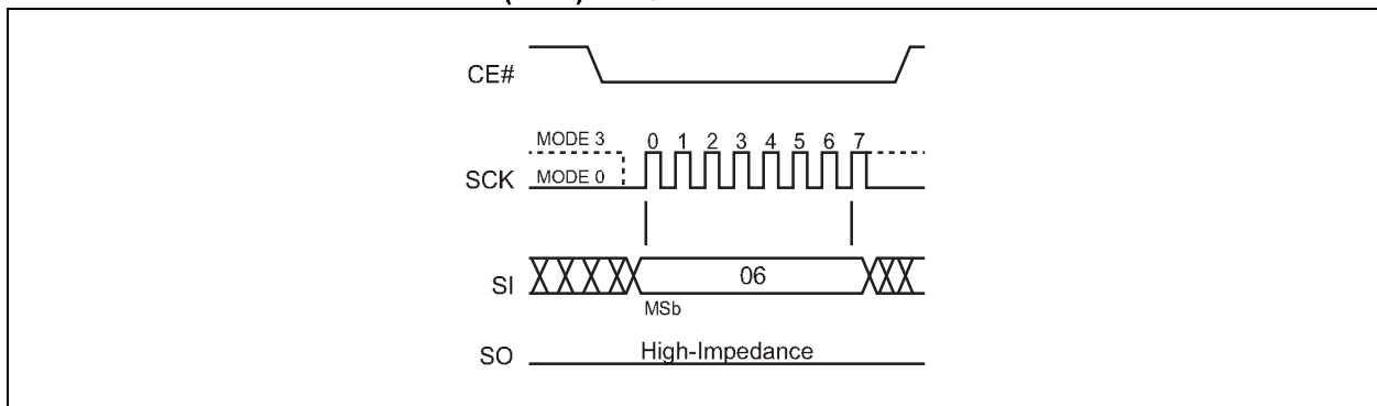
FIGURE 5-14: WRITE ENABLE (WREN) SEQUENCE
