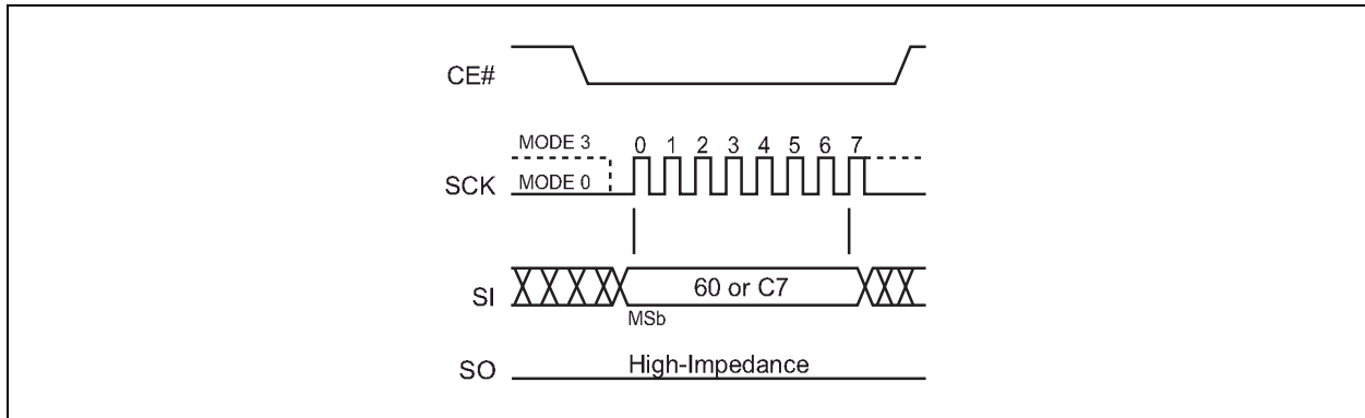
FIGURE 5-11: CHIP-ERASE SEQUENCE
