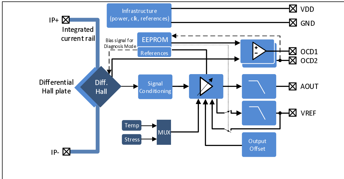
Figure 2 Block Diagram
