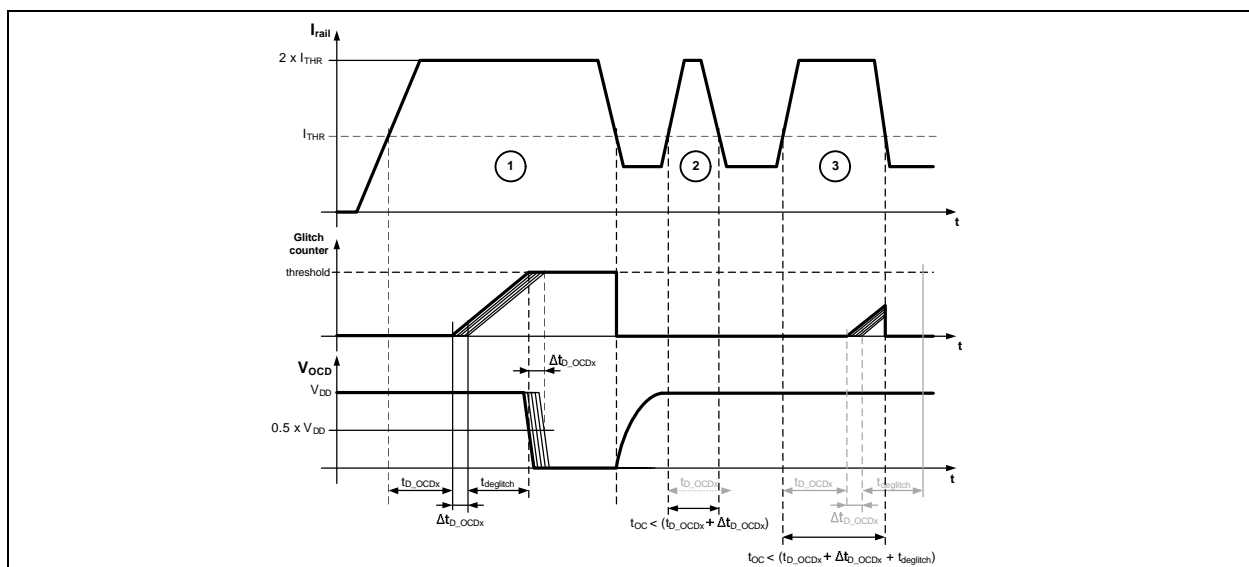
Figure 4 Fast over-current detection output timing
