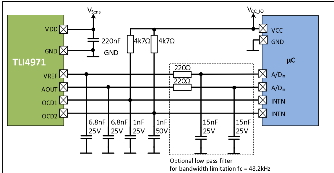
Figure 7 Application circuit with external components
