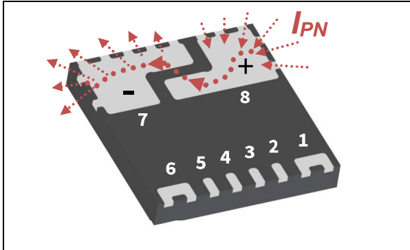
Figure 1 Pin layout PG-TISON-8-5
