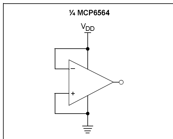
FIGURE 4-11: Unused Comparators.
