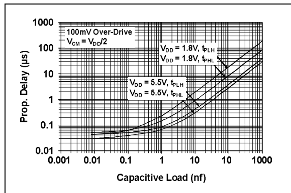
FIGURE 2-31: Propagation Delay vs. Capacitive Load.
