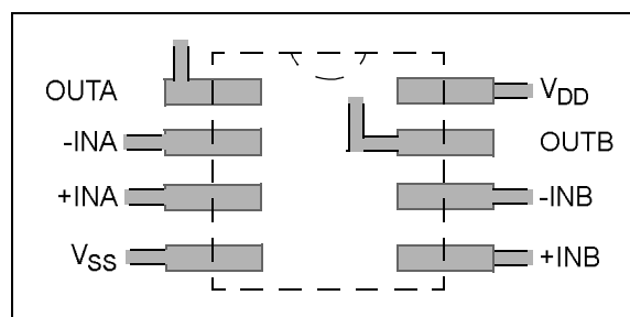
FIGURE 4-10: Recommended Layout.
