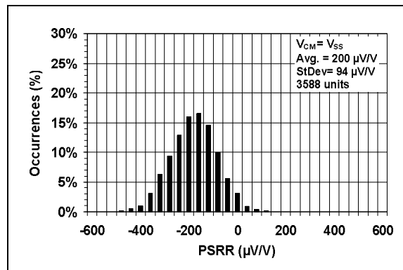
FIGURE 2-34: Power Supply Rejection Ratio (PSRR).
