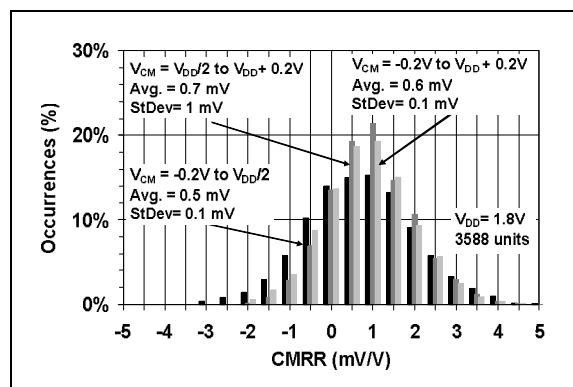
FIGURE 2-35: Common-Mode Rejection Ratio (CMRR).
