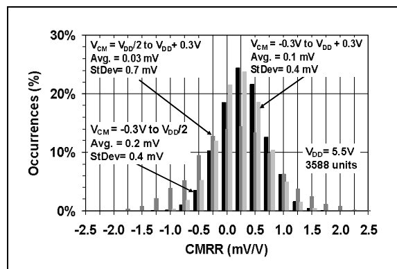
FIGURE 2-36: Common-Mode Rejection Ratio (CMRR).
