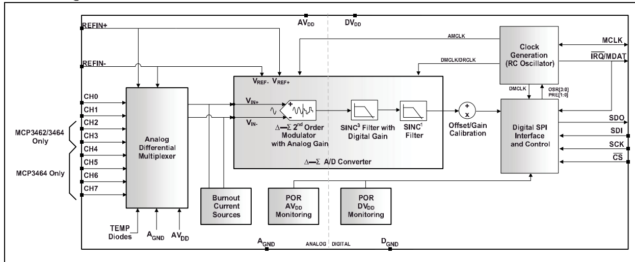
Block Diagram of MCP3461/2/4 Devices
