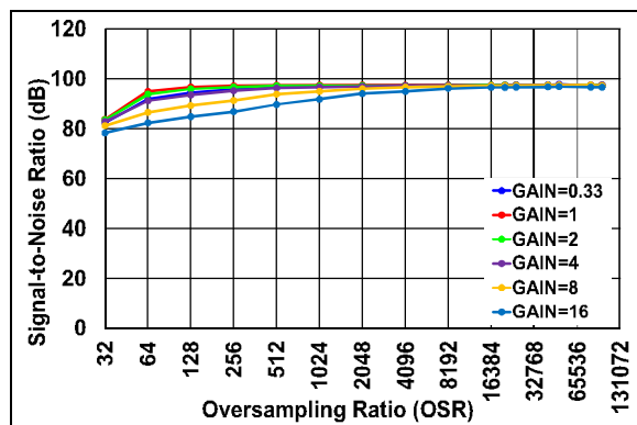
FIGURE 2-8: SNR vs. OSR.
