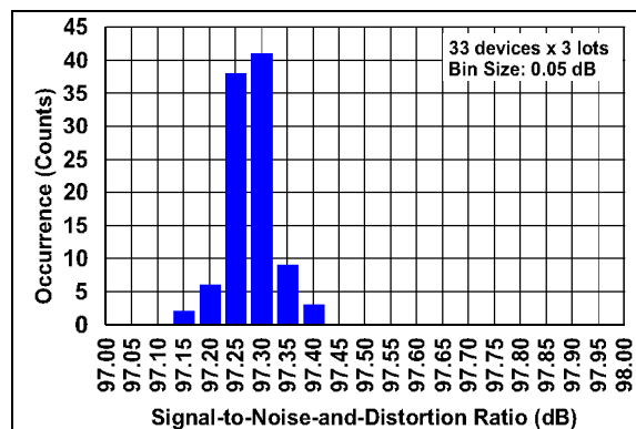
FIGURE 2-11: SINAD Distribution Histogram.
