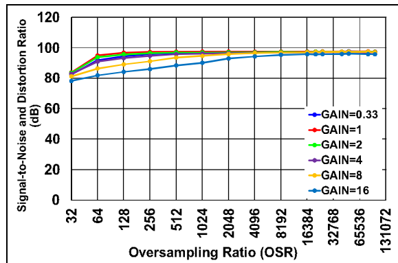
FIGURE 2-7: SINAD vs. OSR.
