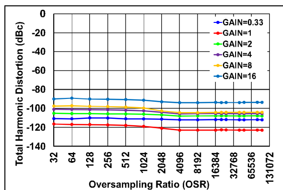
FIGURE 2-9: THD vs. OSR.
