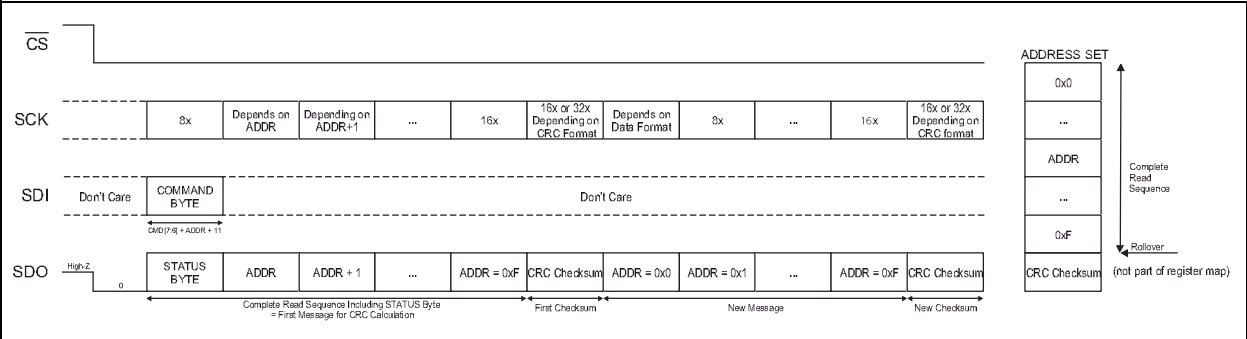
FIGURE 6-13: SPI Incremental Read with Communication CRC Enabled.
