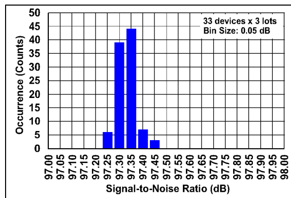
FIGURE 2-12: SNR Distribution Histogram.
