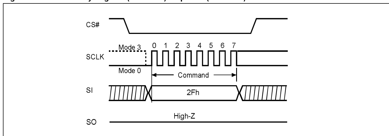
Figure 66. Write Security Register (WRSCUR) Sequence (SPI Mode)
