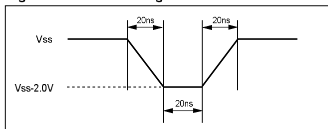
Figure 84. Maximum Negative Overshoot Waveform
