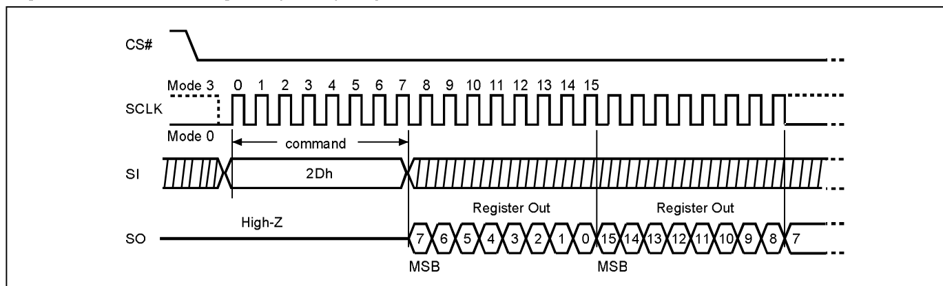
Figure 70. Read Lock Register (RDLR) Sequence
