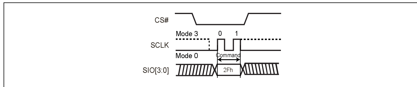
Figure 67. Write Security Register (WRSCUR) Sequence (QPI Mode)
