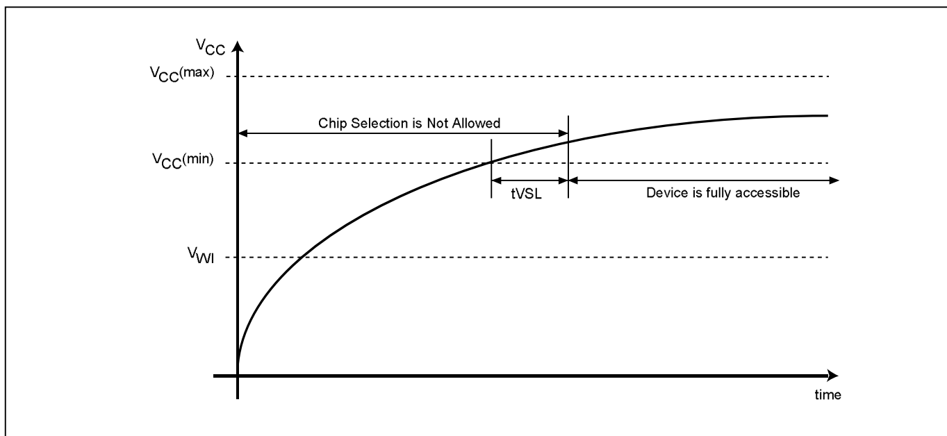
Figure 90. Power-up Timing
