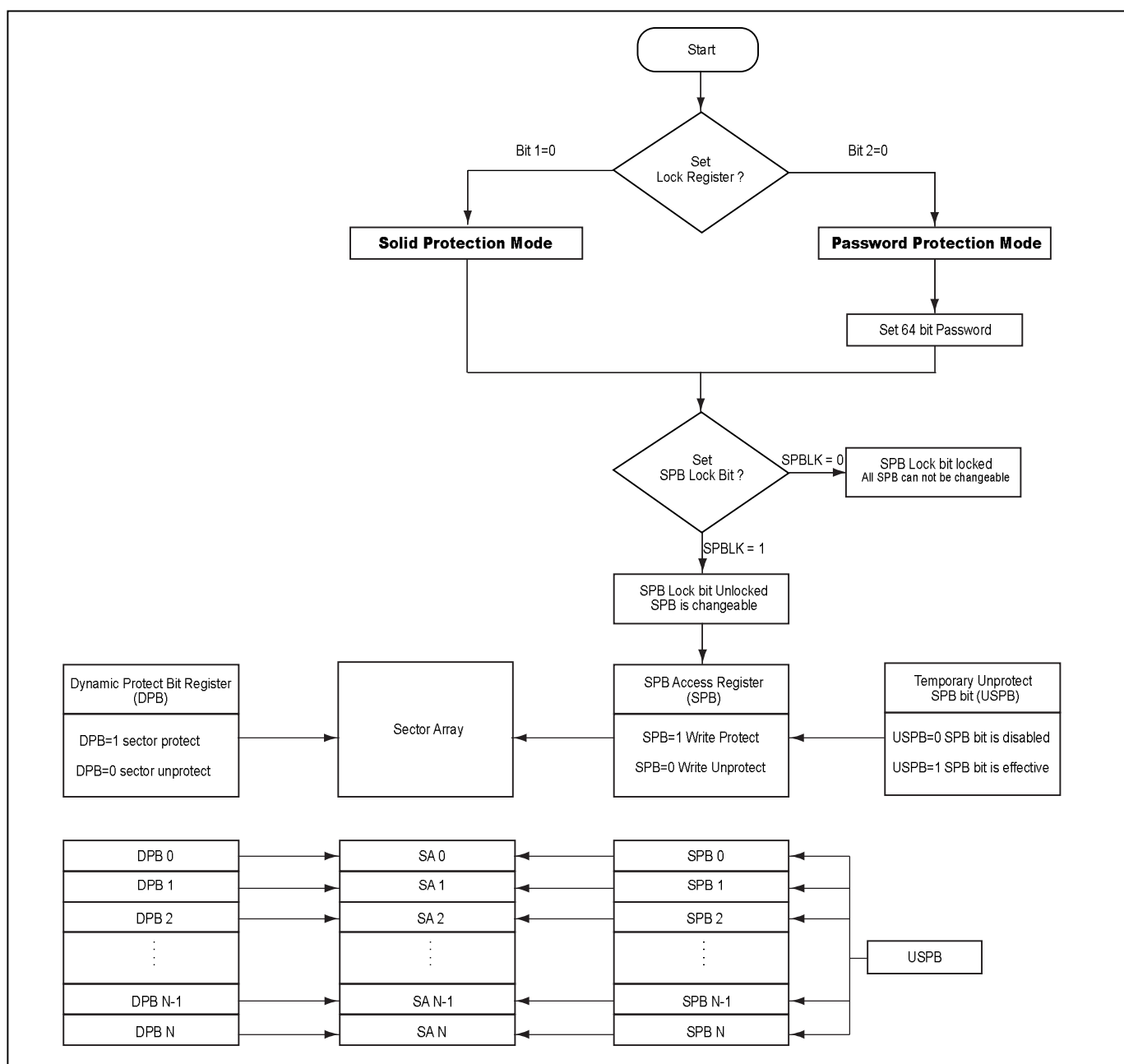
Figure 69. Advanced Sector Protection Overview
