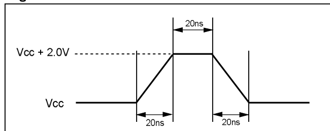
Figure 85. Maximum Positive Overshoot Waveform
