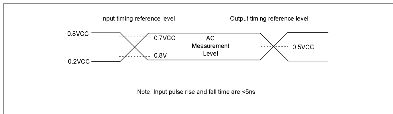
Figure 86. INPUT TEST WAVEFORMS AND MEASUREMENT LEVEL
