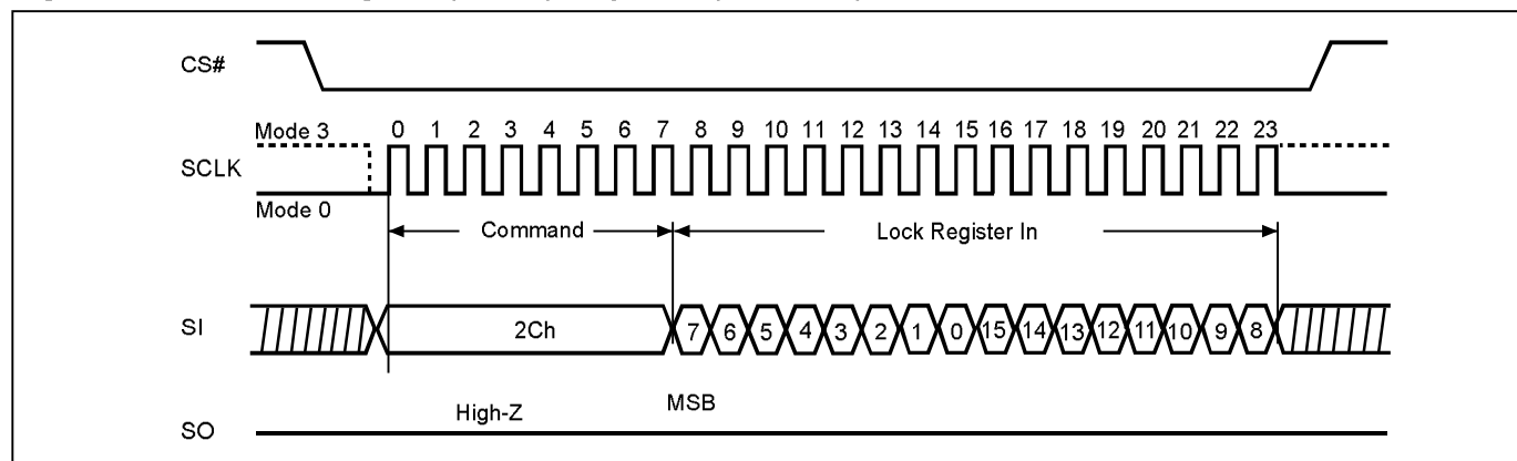
Figure 71. Write Lock Register (WRLR) Sequence (SPI Mode)
