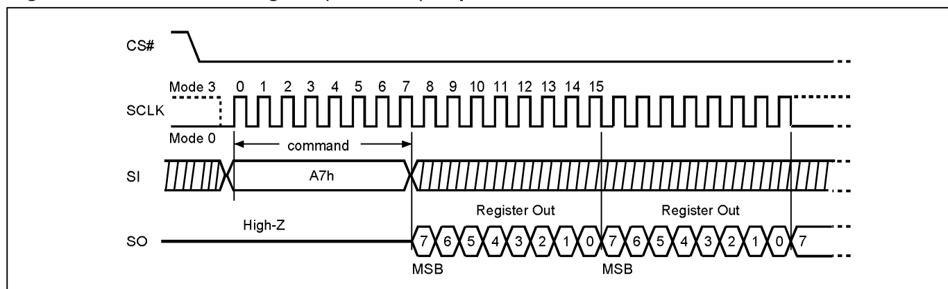
Figure 73. Read SPB Lock Register (RDSPBLK) Sequence
