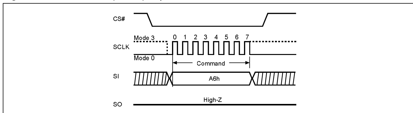
Figure 72. SPB Lock Bit Set (SPBLK) Sequence
