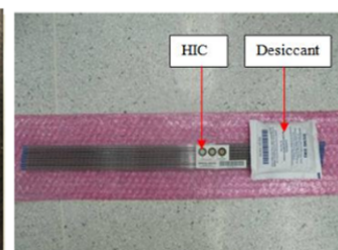
Fig-2 (Attach HIC & Desiccant)
