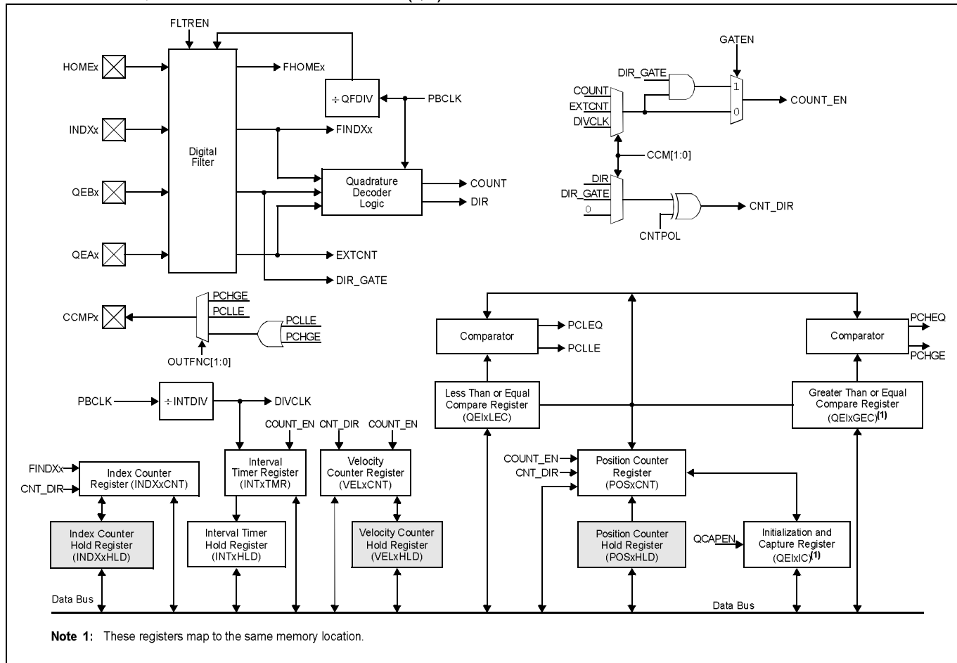
FIGURE 15-2: QUADRATURE ENCODER INTERFACE (QEI) MODULE BLOCK DIAGRAM
