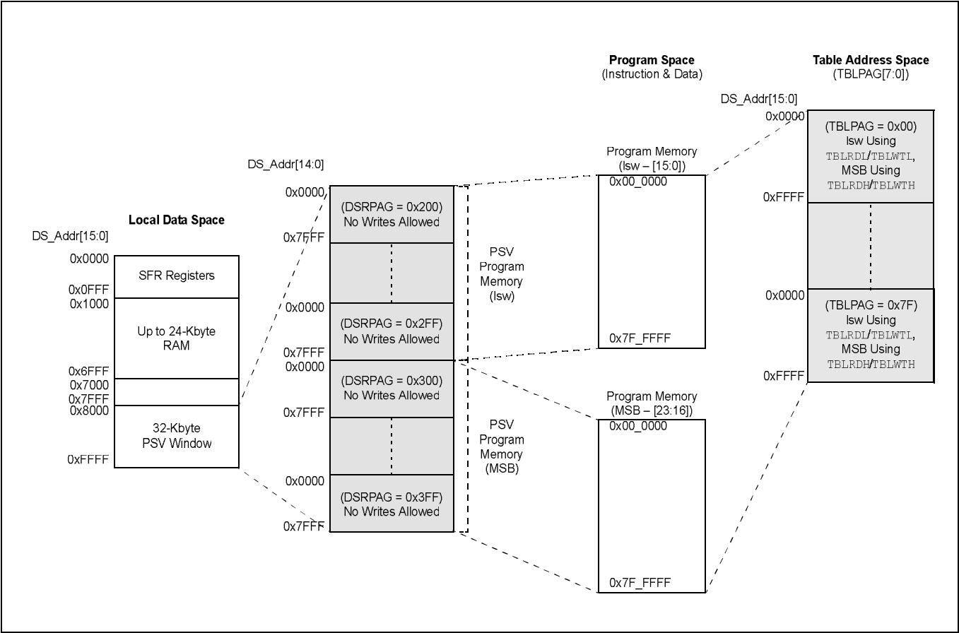
FIGURE 4-12: PAGED DATA MEMORY SPACE
