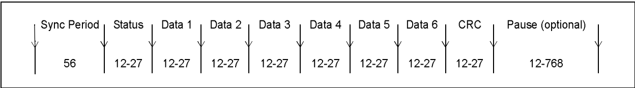
FIGURE 20-2: SENTx PROTOCOL DATA FRAMES
