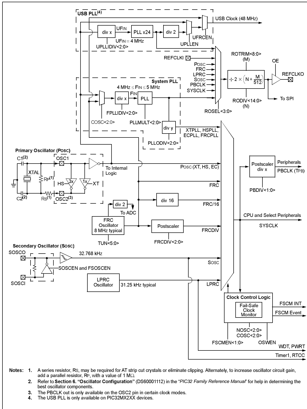
FIGURE 8-1: OSCILLATOR DIAGRAM
