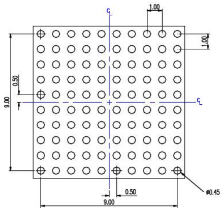
RECOMMENDED LAND PATTERN NOTE 1
