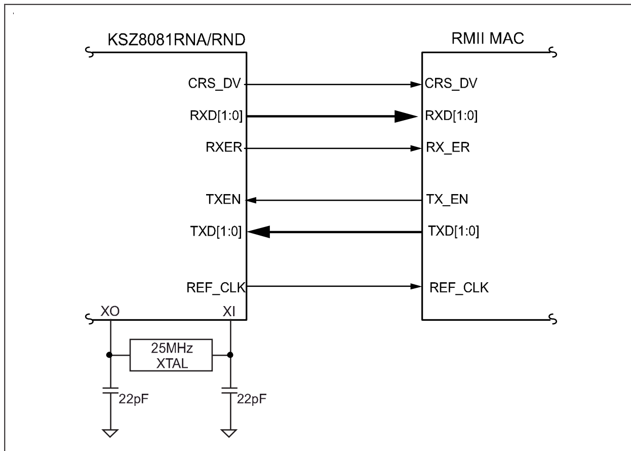
FIGURE 3-2: KSZ8081RNA/RND RMII INTERFACE (RMII - 25 MHZ CLOCK MODE)
