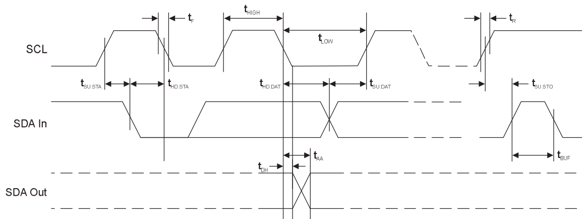
Figure 4-1. Bus Timing
