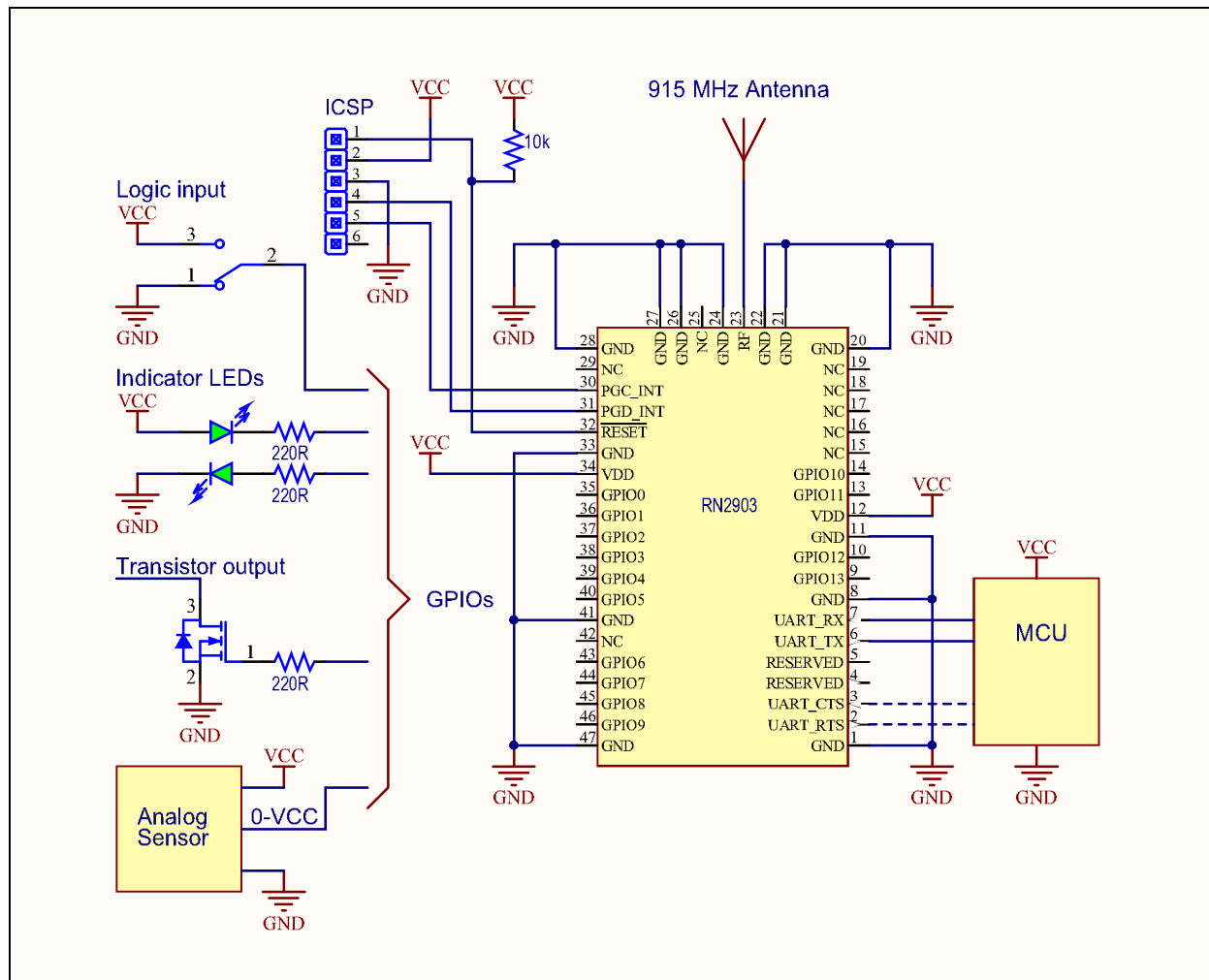
FIGURE 3-1: HARDWARE CONNECTIONS
