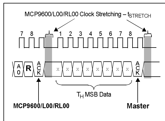
FIGURE 4-2: Clock Stretching.
