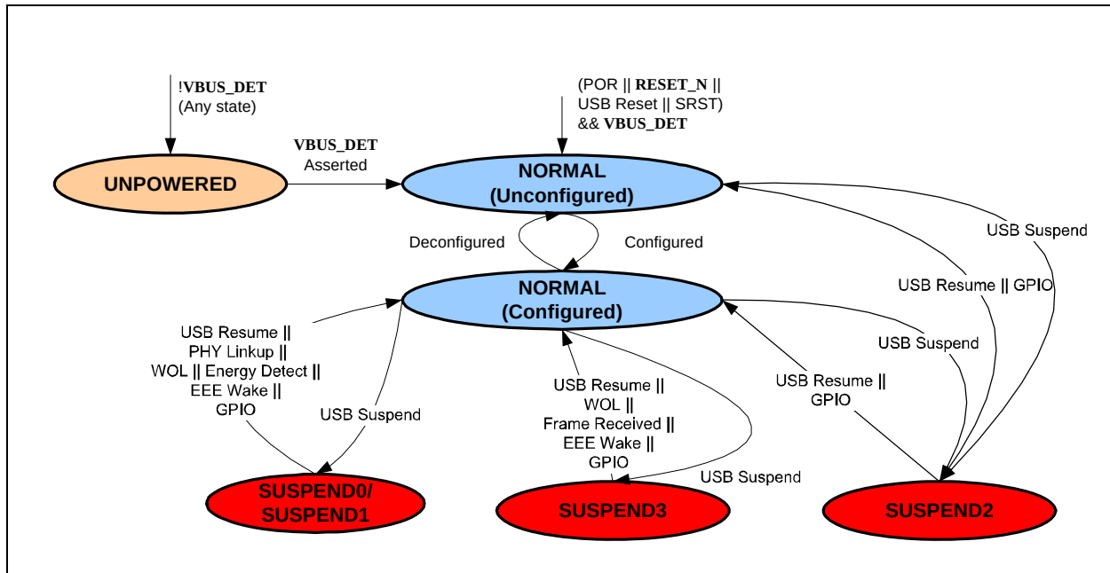
FIGURE 12-1: POWER STATES
