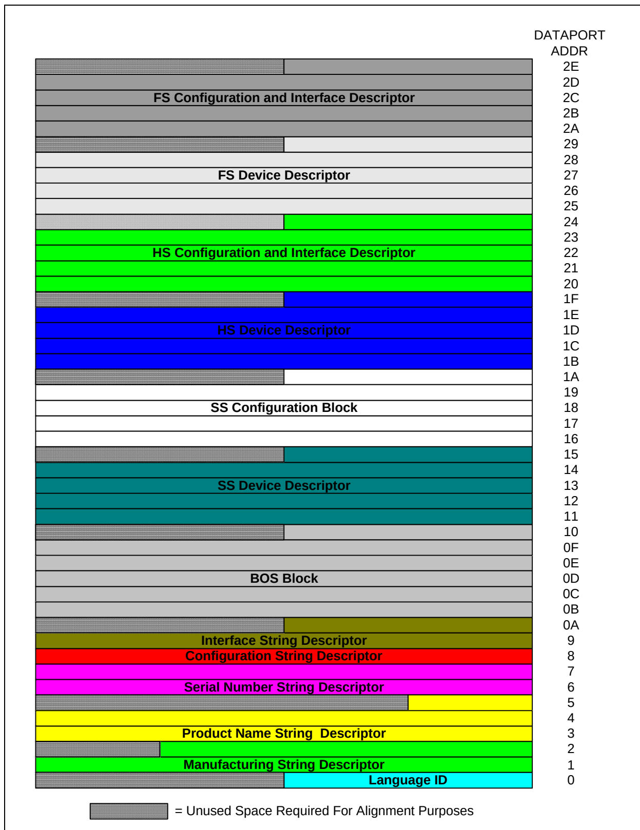
FIGURE 9-9: DESCRIPTOR RAM EXAMPLE
