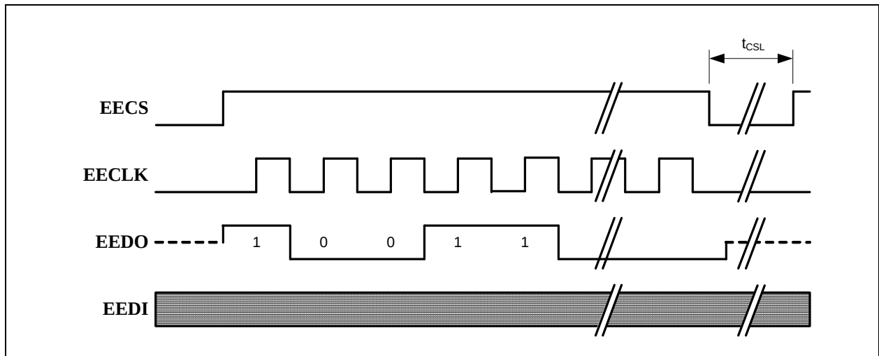
FIGURE 9-5: EEPROM EWEN CYCLE
