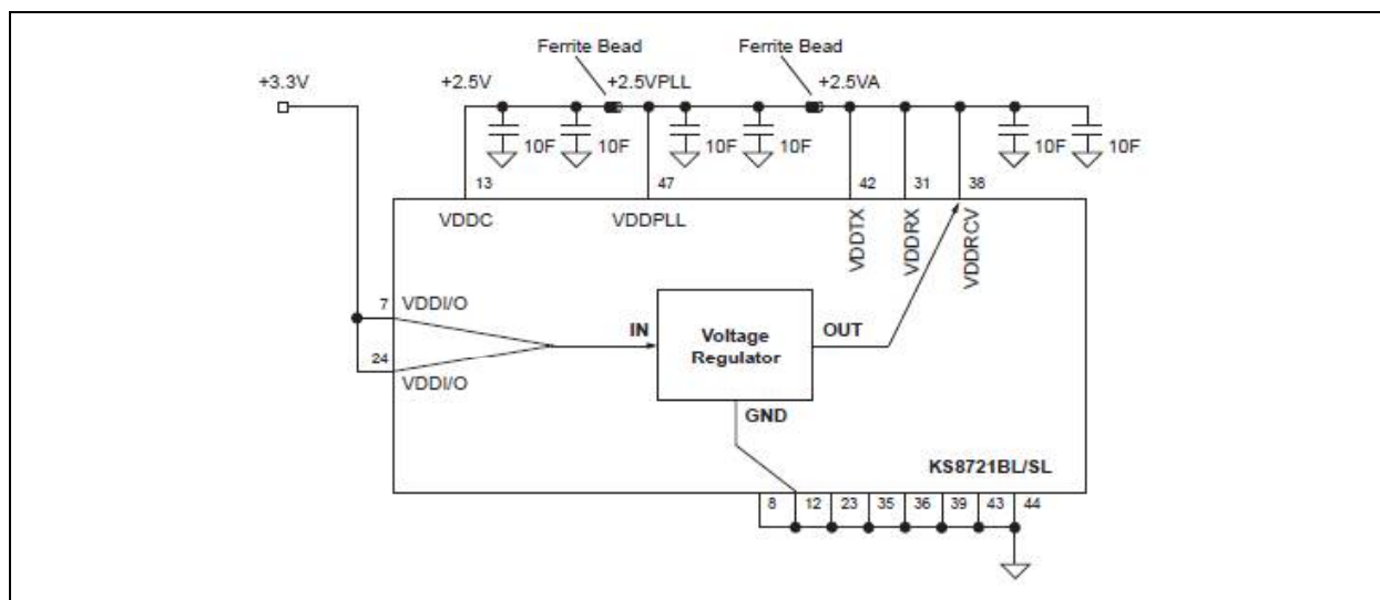
FIGURE 3-4: CIRCUIT DESIGN
