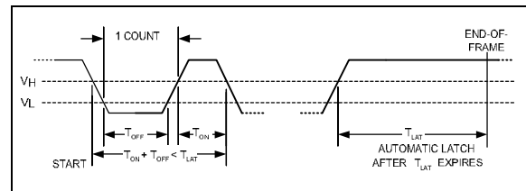
FIGURE 5-2: Data Word Pulse Timing.
