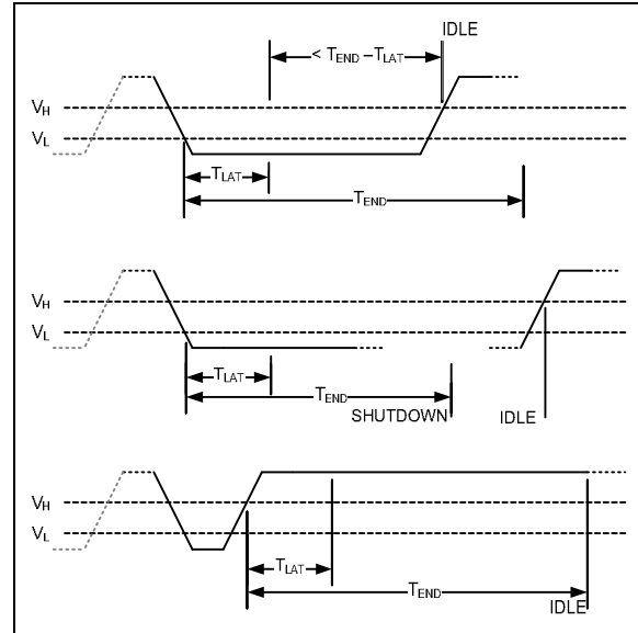
FIGURE 5-1: Abort, Shutdown and Idle Timing Waveforms.
