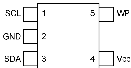
5-lead SOT23 (1)
