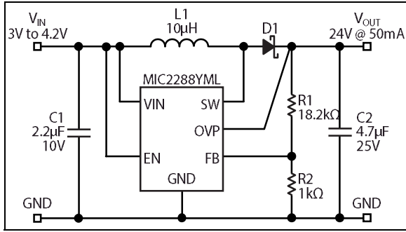
FIGURE 6-5: 3.0V to 4.2V V_{IN} to 24V _{OUT} @ 50 mA.
