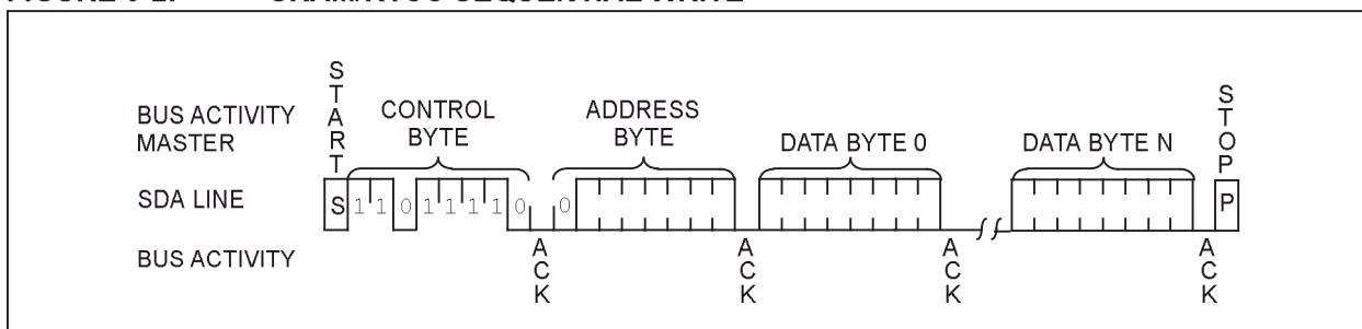
FIGURE 6-2: SRAM/RTCC SEQUENTIAL WRITE
