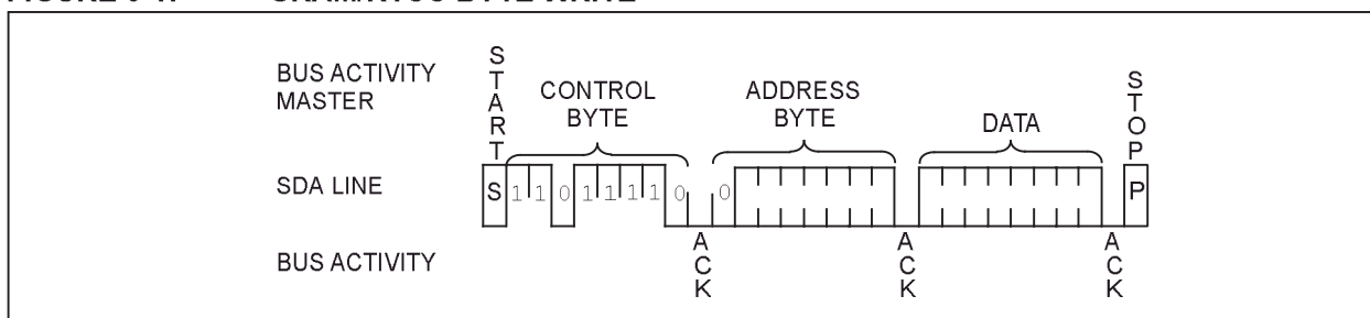
FIGURE 6-1: SRAM/RTCC BYTE WRITE
